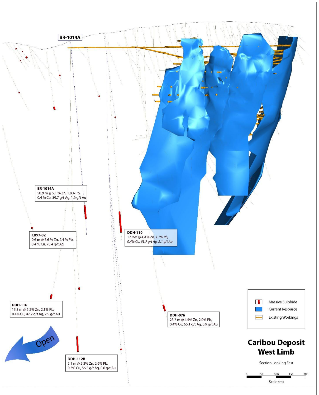
Figure 1: 3D long section of Caribou deposit west limb illustrating the location of BR-1014A intercept.
