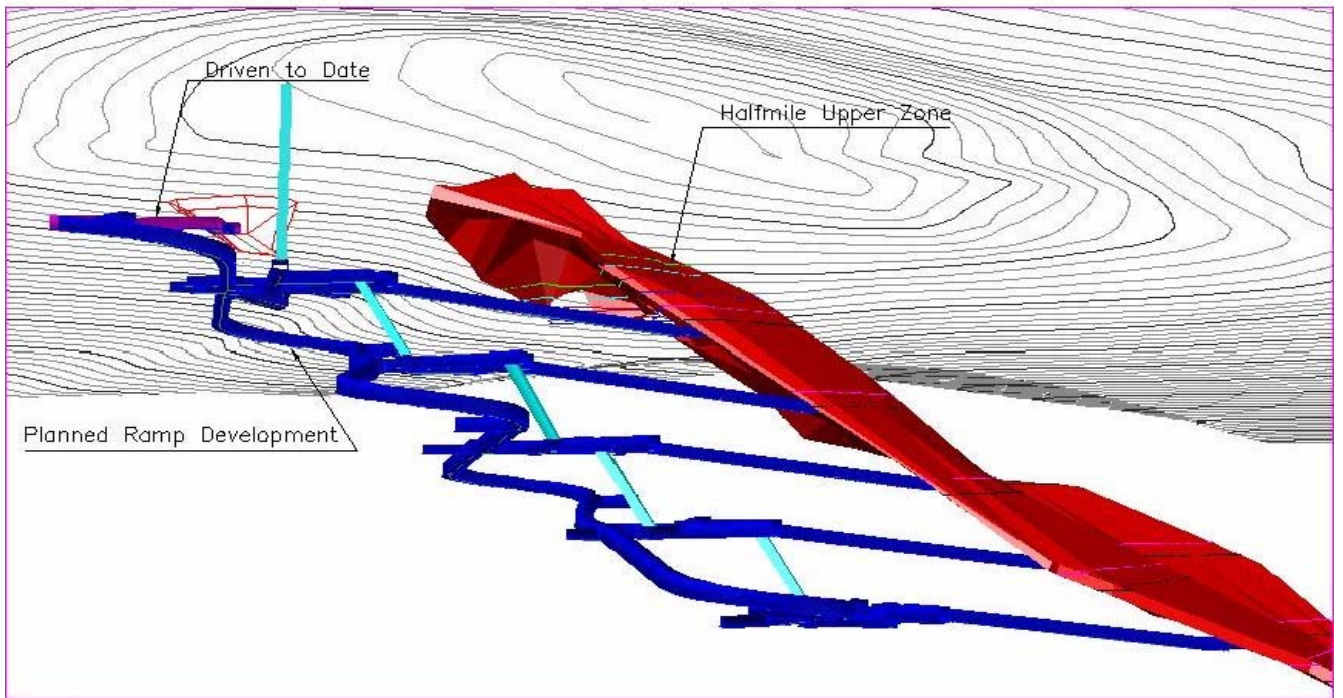
Figure 2: Halfmile Upper Zone Mine Development Plan
