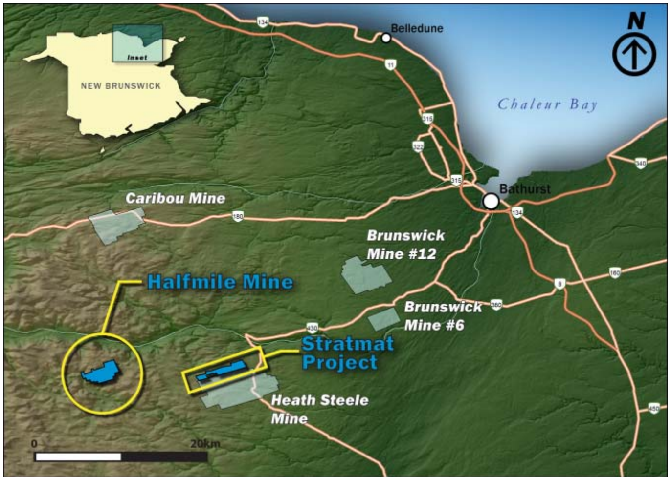
Figure 3: Stratmat deposit and Halfmile Mine location map, northeastern New Brunswick
