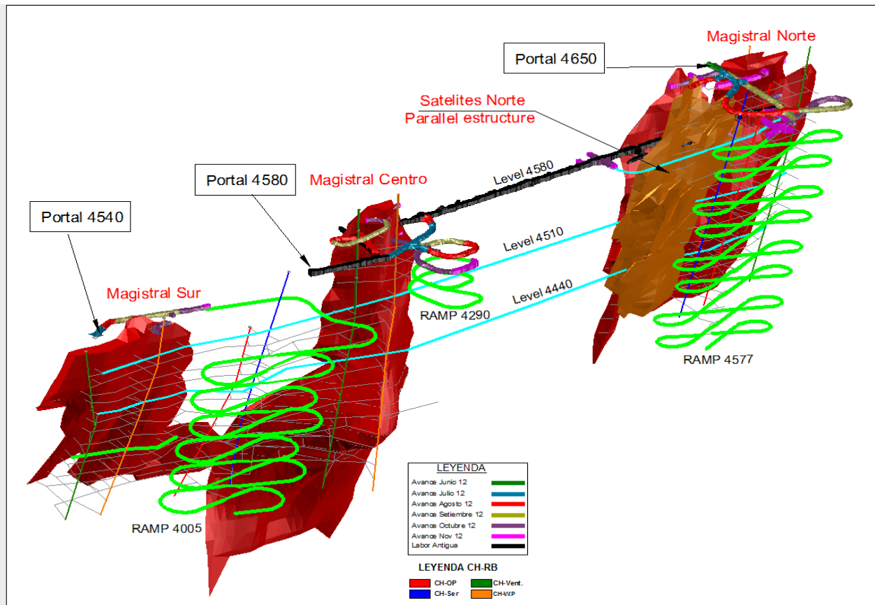
Figure 3: Underground development progress and plan on Magistral North, Central and South deposits at Santander Mine
