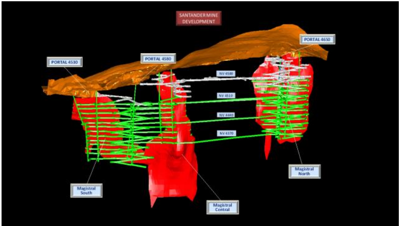
Figure 1: Current Santander Mine underground workings (white) and planned development (green).
