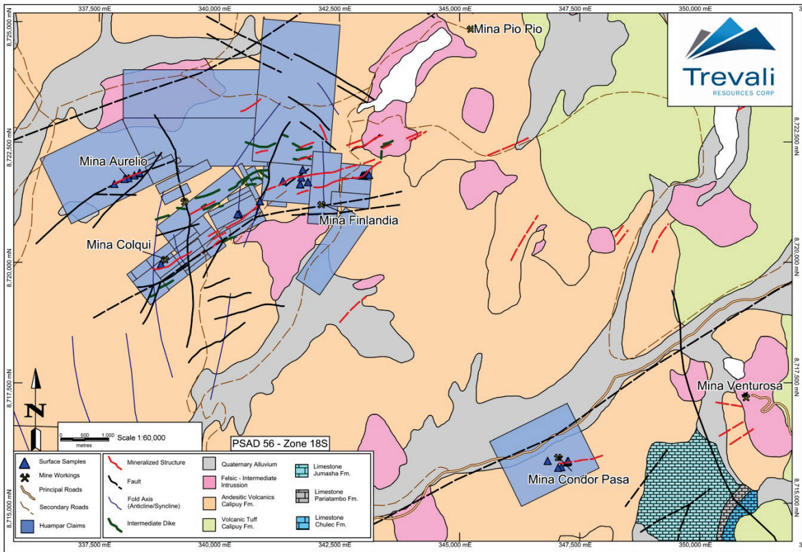
Figure 1: Simplified geological map showing the Huampar property and location of due diligence samples.
