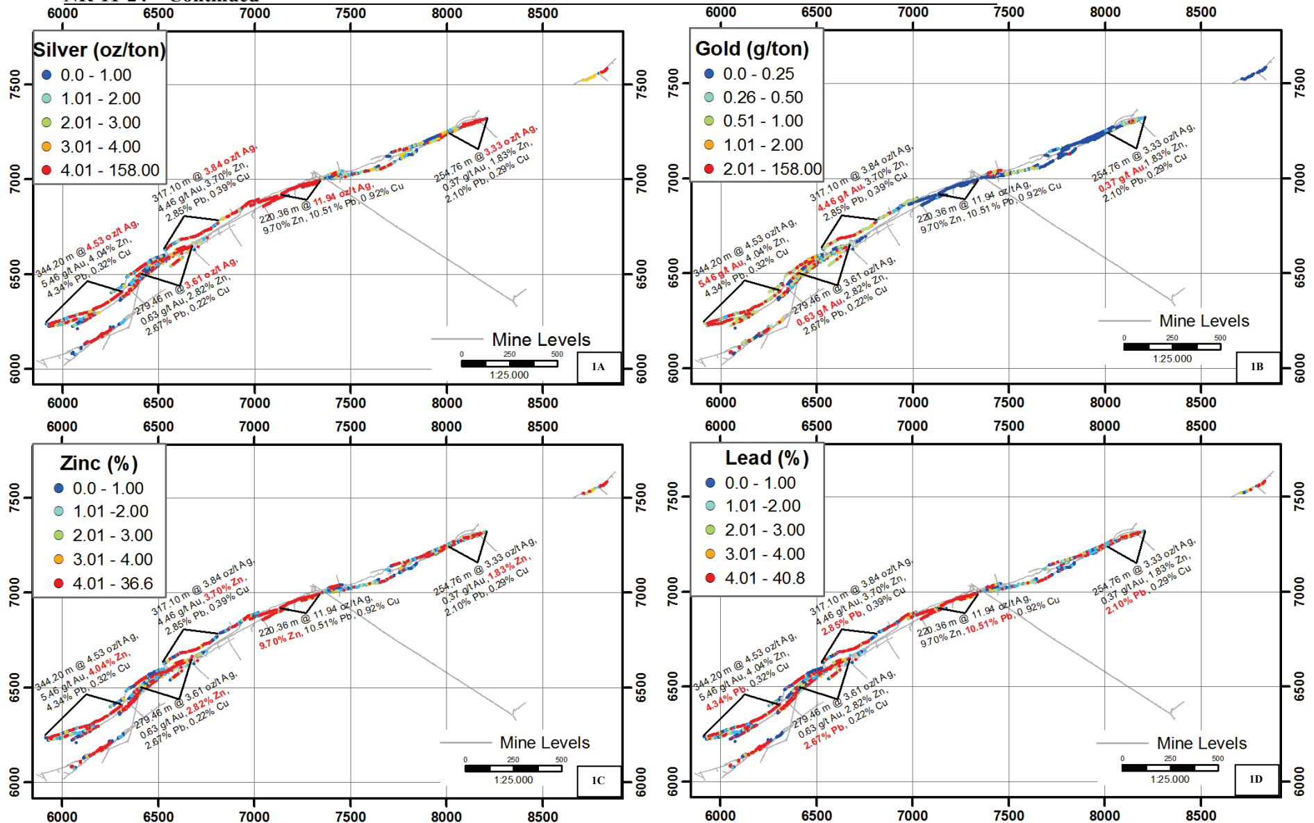
Figure 2: Composite level-plan of levels 428, 421, 416, and 412 showing the distribution of silver (1A), gold (1B), zinc (1C) and lead (1D)
