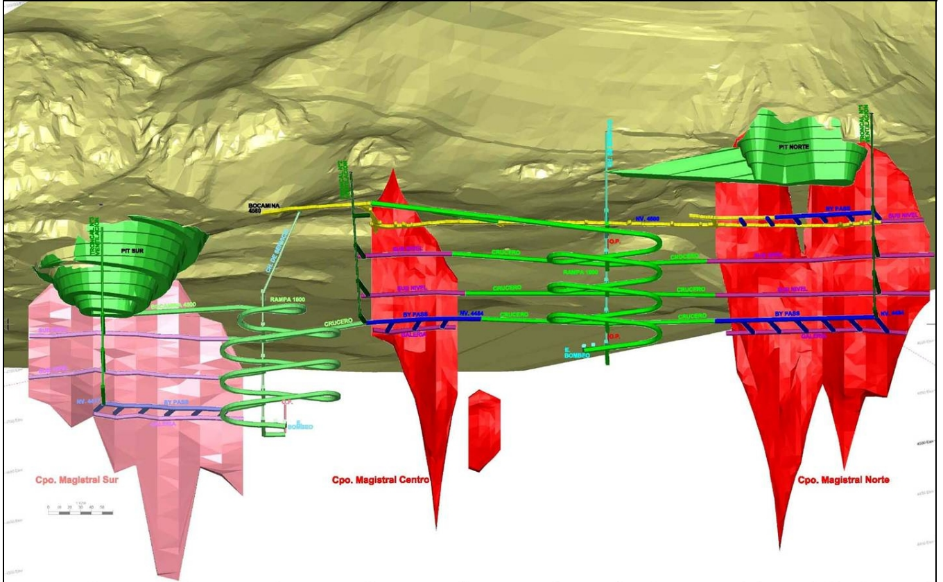
Figure 1. Mine plan for the Magistral South, Central and North deposits from the joint Trevali-Glencore internal mine development study indicating planned open pits on the South and North deposits, and underground development modeling.
