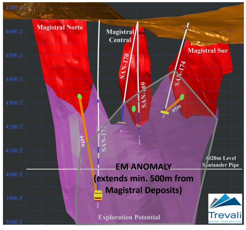
Figure 1: 3D model of Magistral deposits (red), area of interpreted exploration potential (purple) and recently defined geophysical (EM) anomaly (grey).
