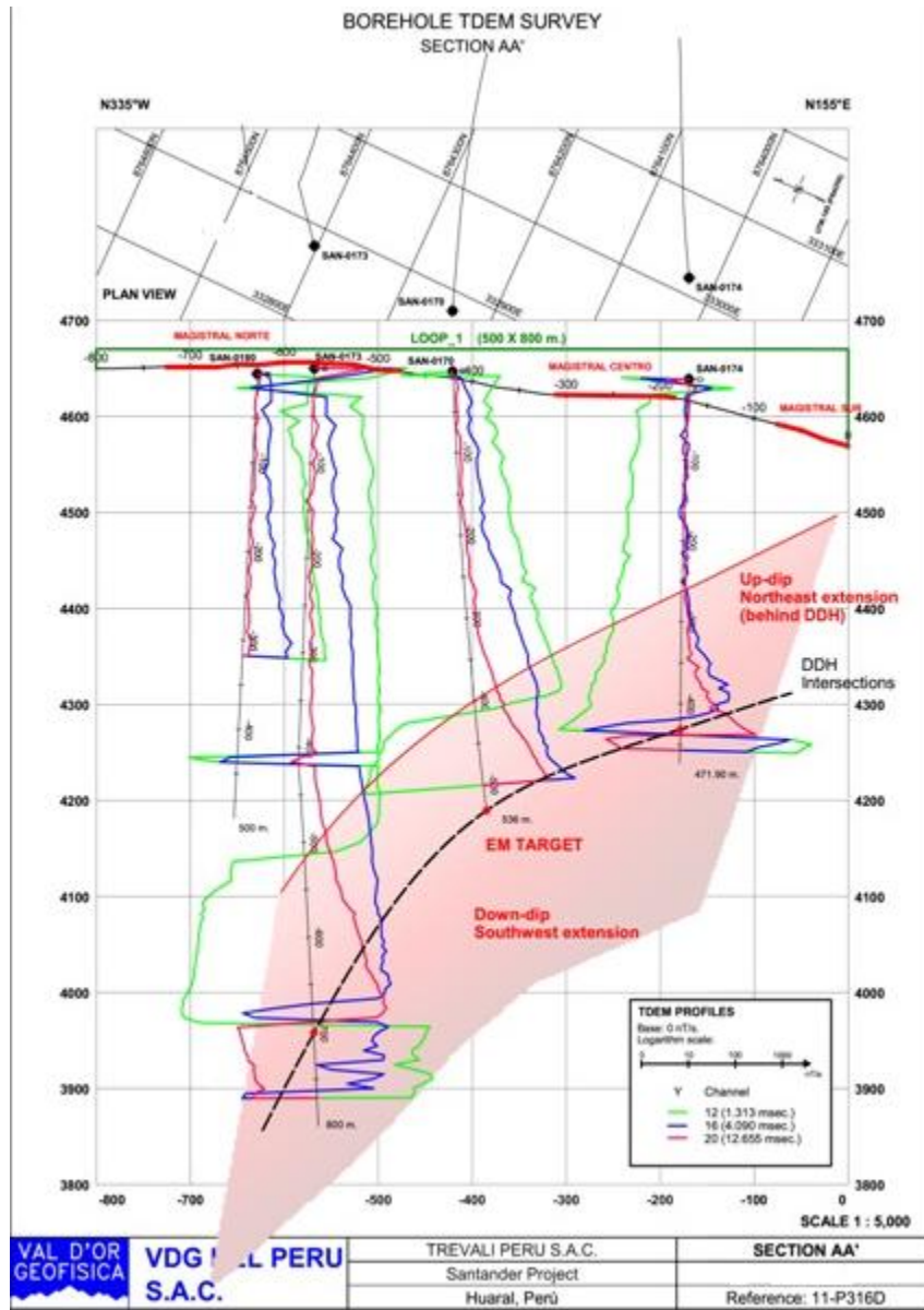
Figure 2: Downhole EM profiles (SAN170, 173 and 173), location of EM Target – after Val D’Or Geophysics.
