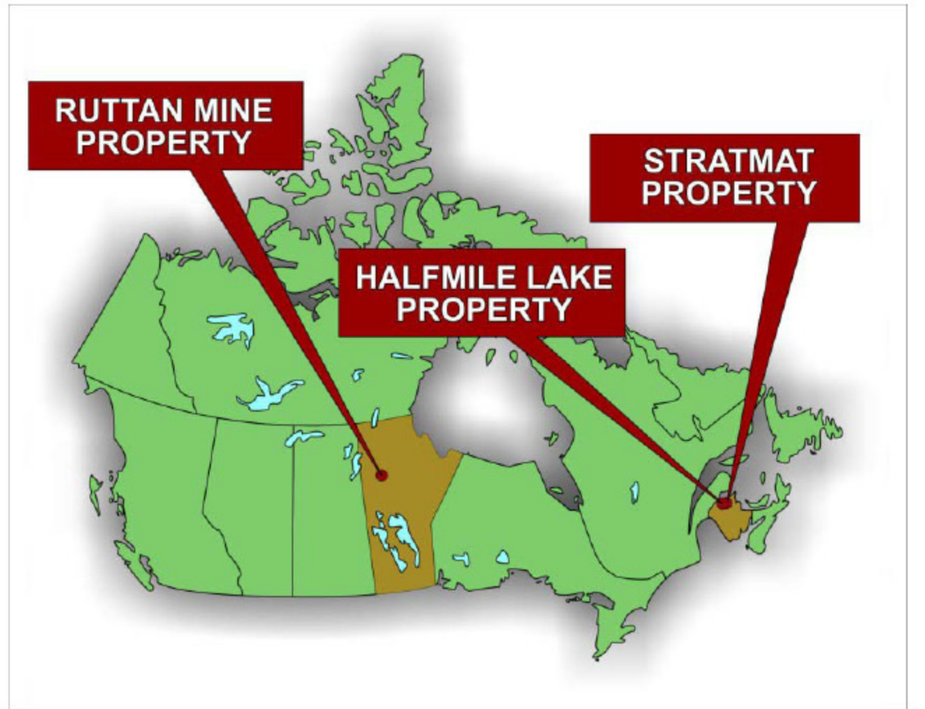
Figure 2. Halfmile, Stratmat and Ruttan location map in Canada
