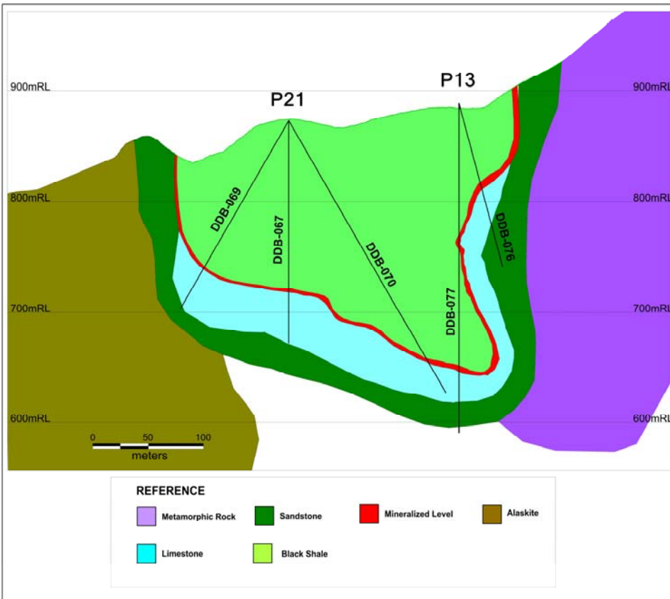
Figure 3 – Cross Section 4
