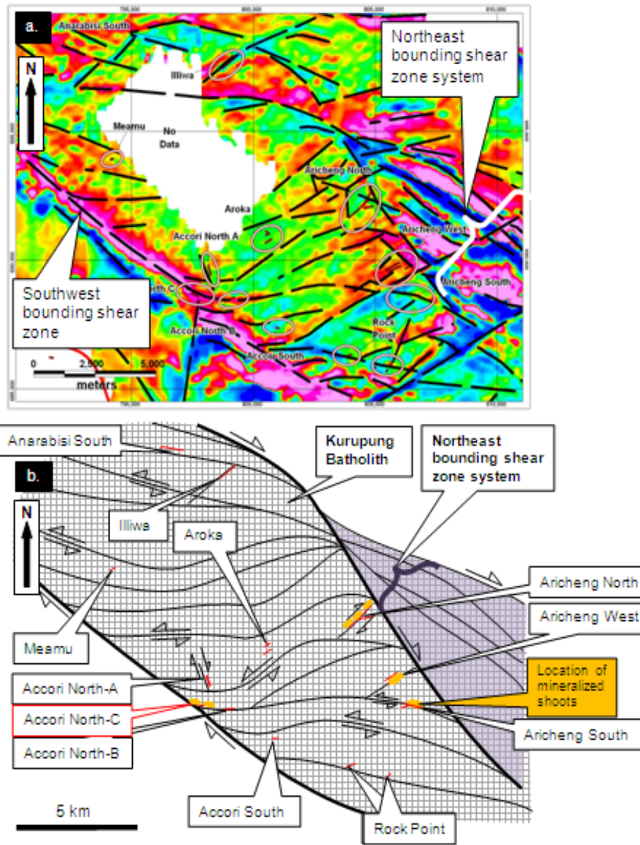
Figure 1 – Map of Magnetic Data and Interpreted Structures in Kurupung Batholith
