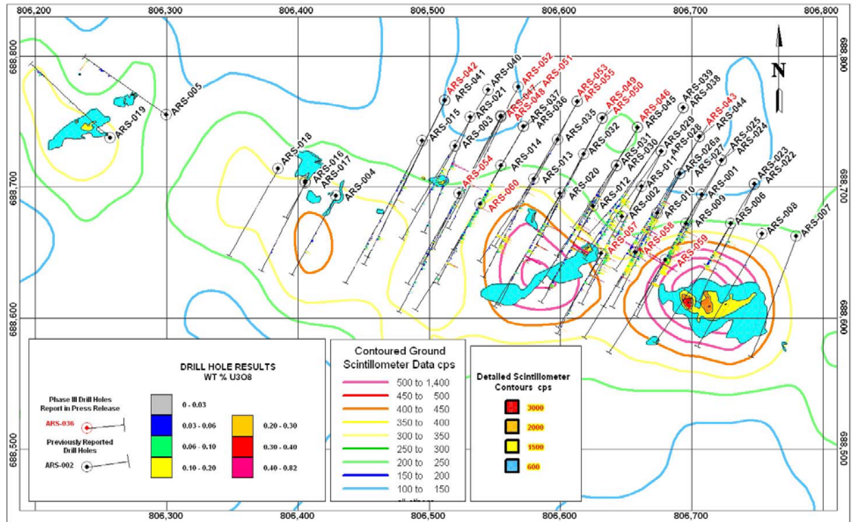
Figure 1. Map showing the ground scintillometer radiometric anomaly at Aricheng South with the location of Phase I, II and previously reported Phase III drill holes labelled in black while the group of 16 Phase III drill holes, whose results are reported here, are labelled in red.
