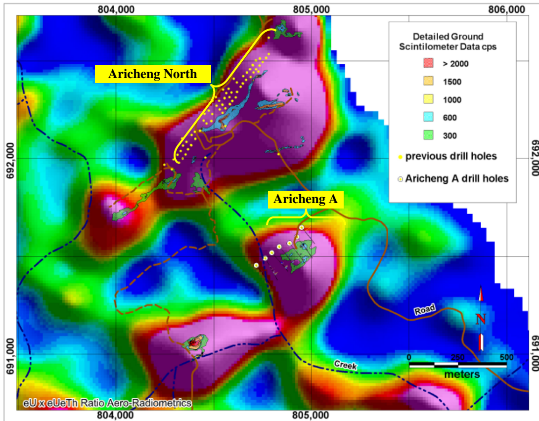
Figure 2 – Drill Hole Locations at Aricheng A
