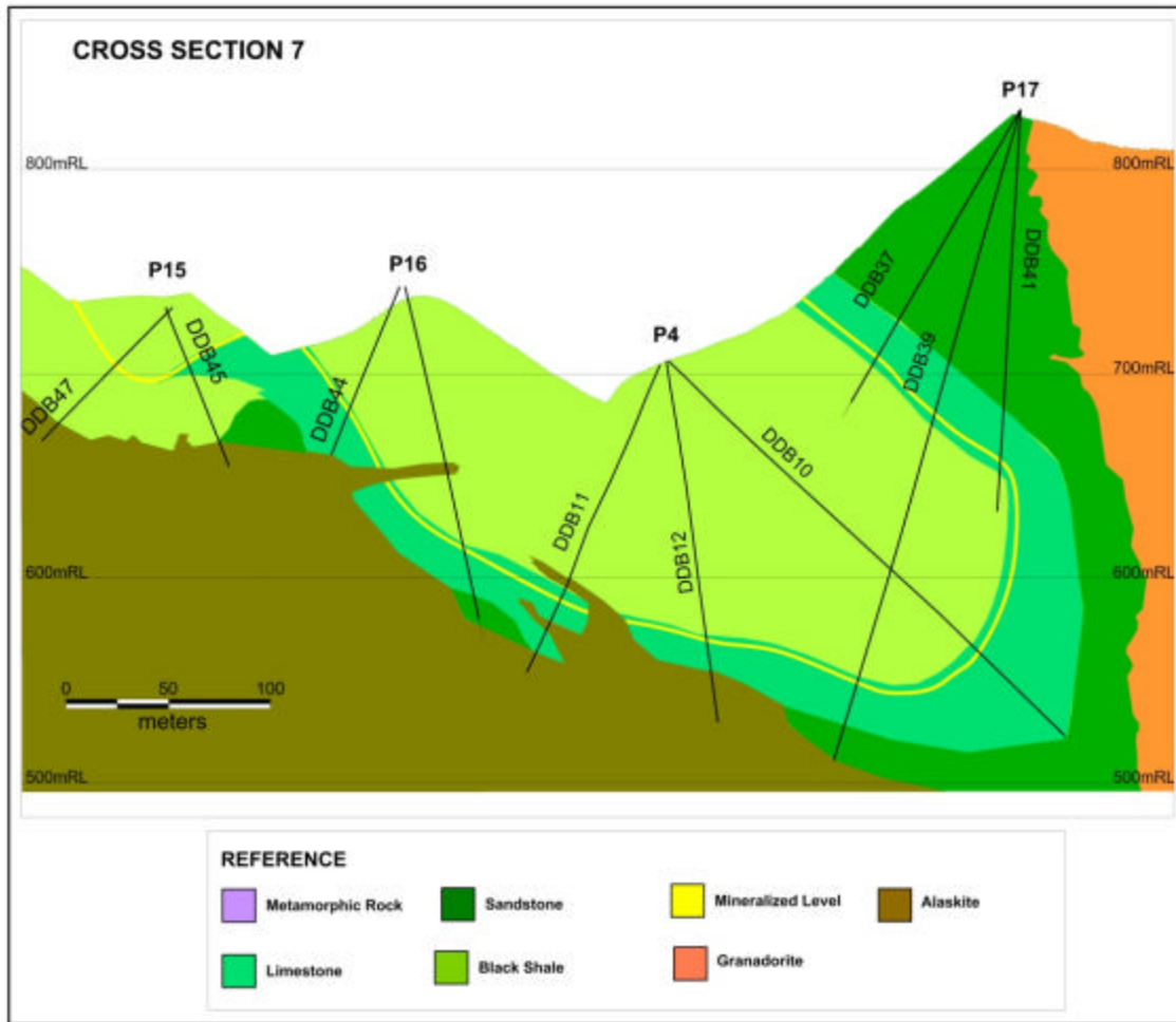
Figure 3 – Cross Section 7
