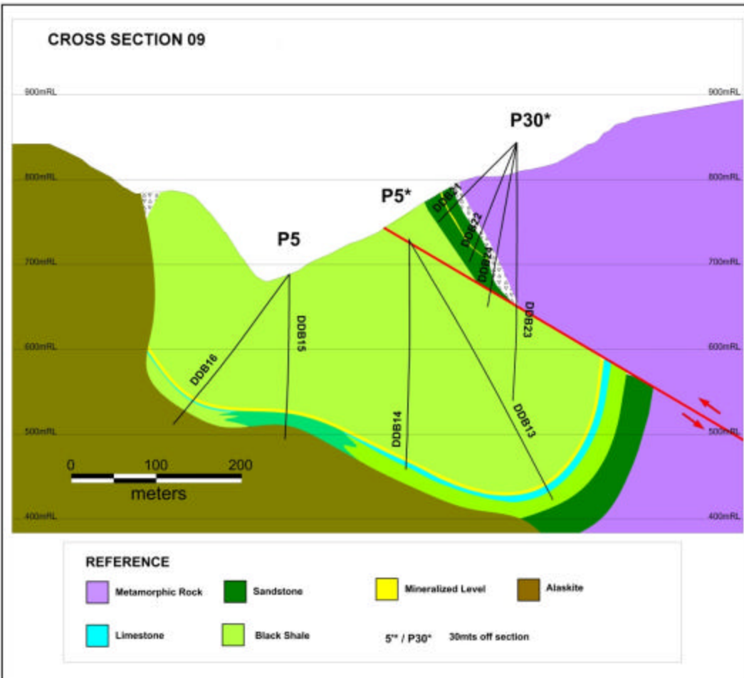
Figure 5 – Cross Section 9
