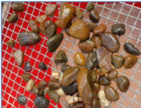
Pebbles rejected from the 15mm screen
