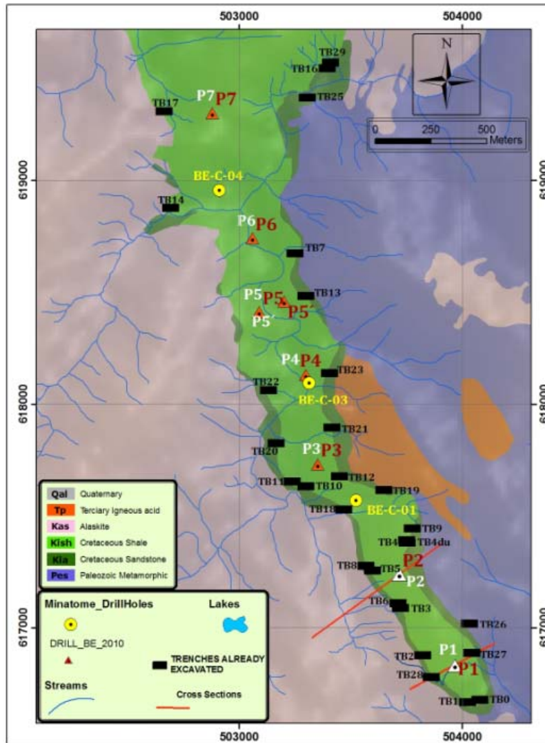
Figure 2 – Drill Locations in the Southern Part of the Fold in the Berlin Project, Colombia
