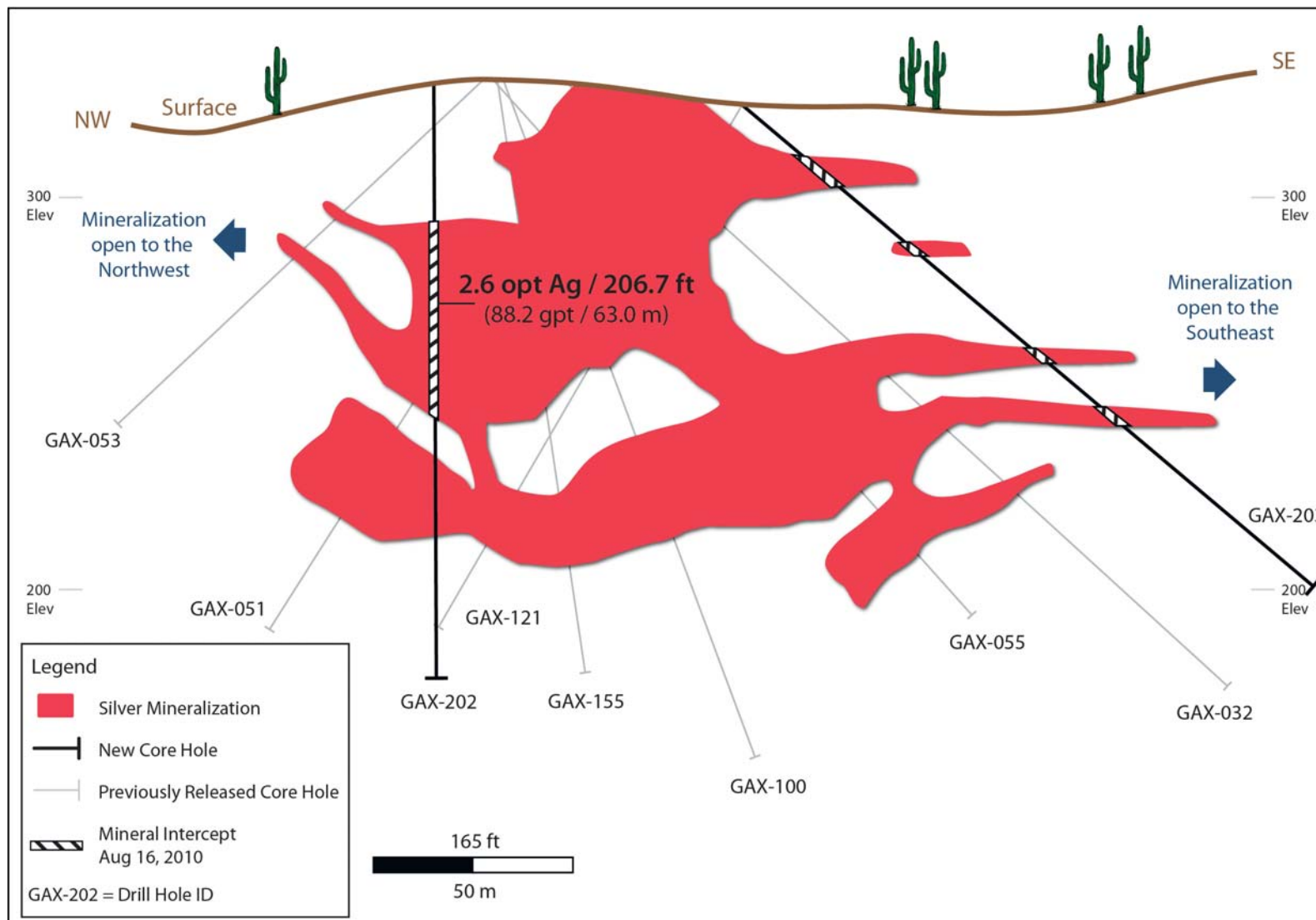
Figure 3 El Gallo Cross Section – Looking East (Section Number: NWSE South 24)
