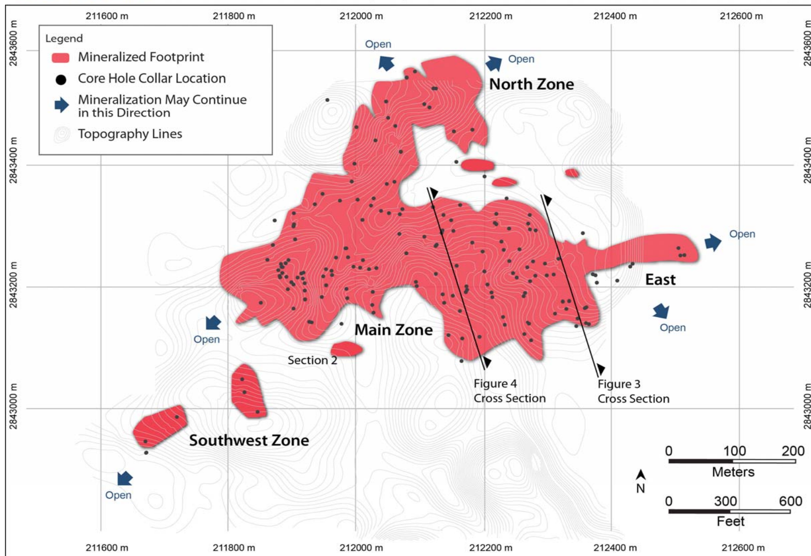
El Gallo Cross Section Locations - Plan (Aerial) View
