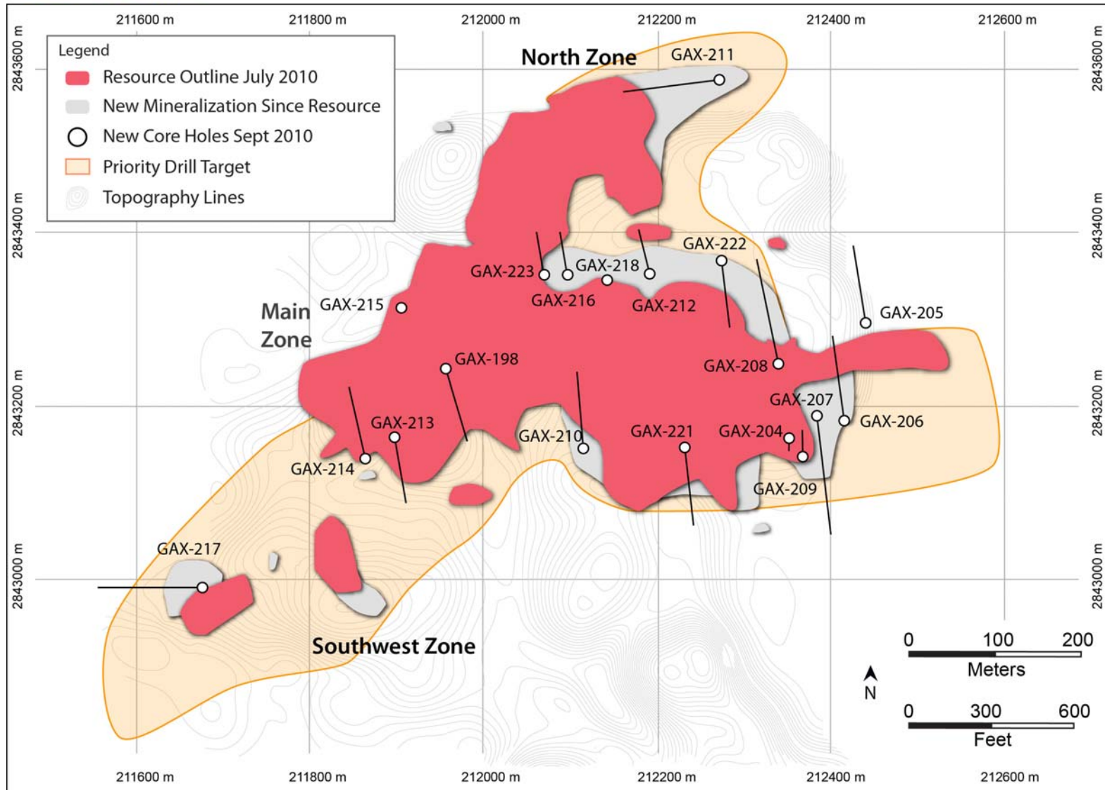
Figure 1 El Gallo - Plan View (Aerial) Map of Drill Hole Locations
