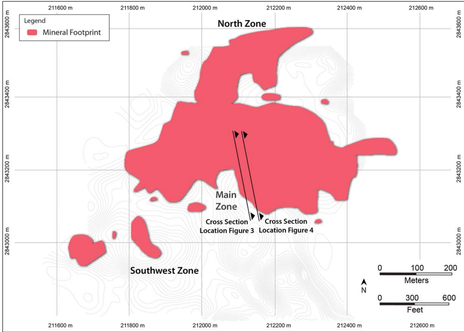
Figure 2 El Gallo - Location of Cross Section
