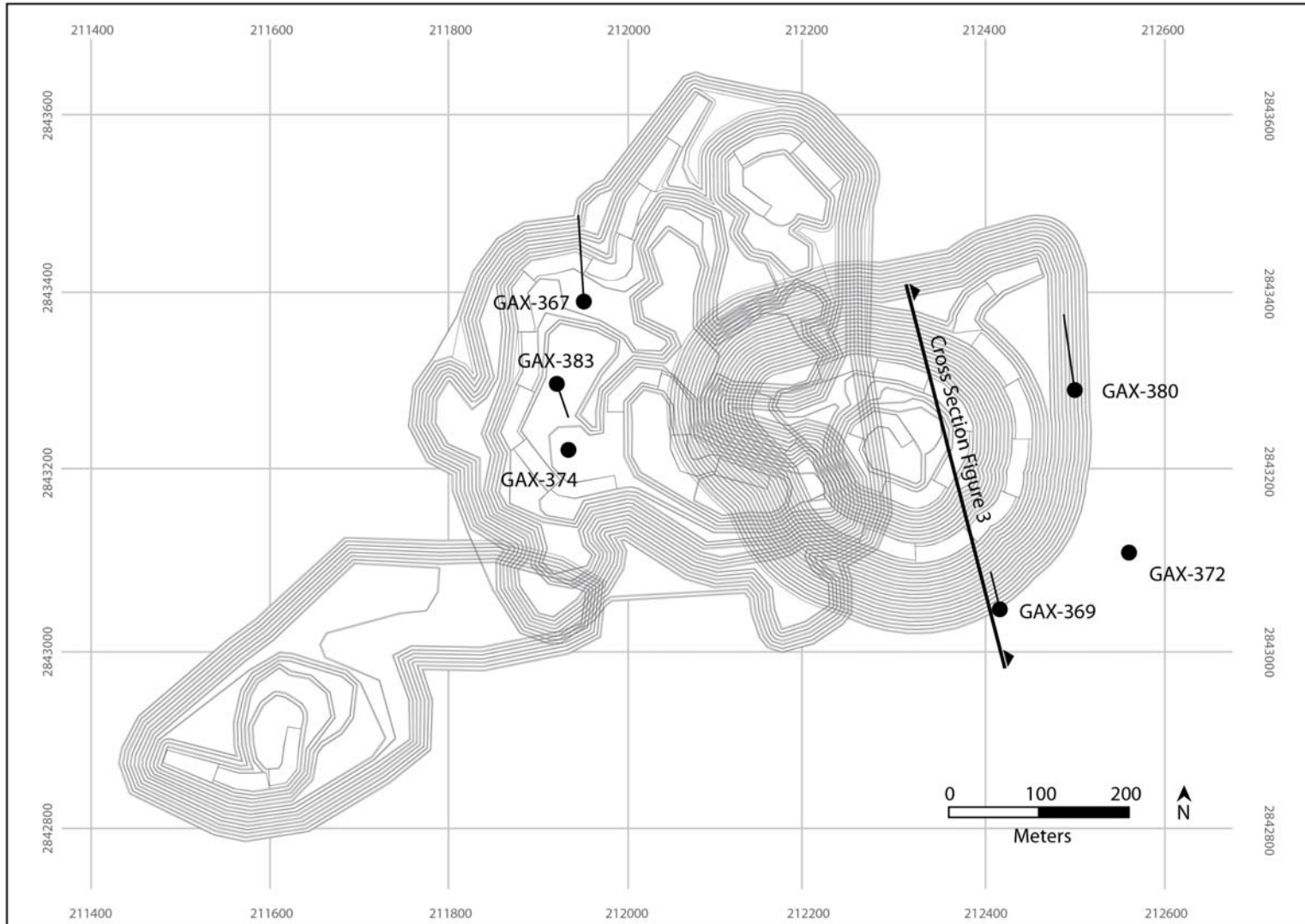
Figure 2 El Gallo Pit Design $18 Silver - Core Hole Locations
