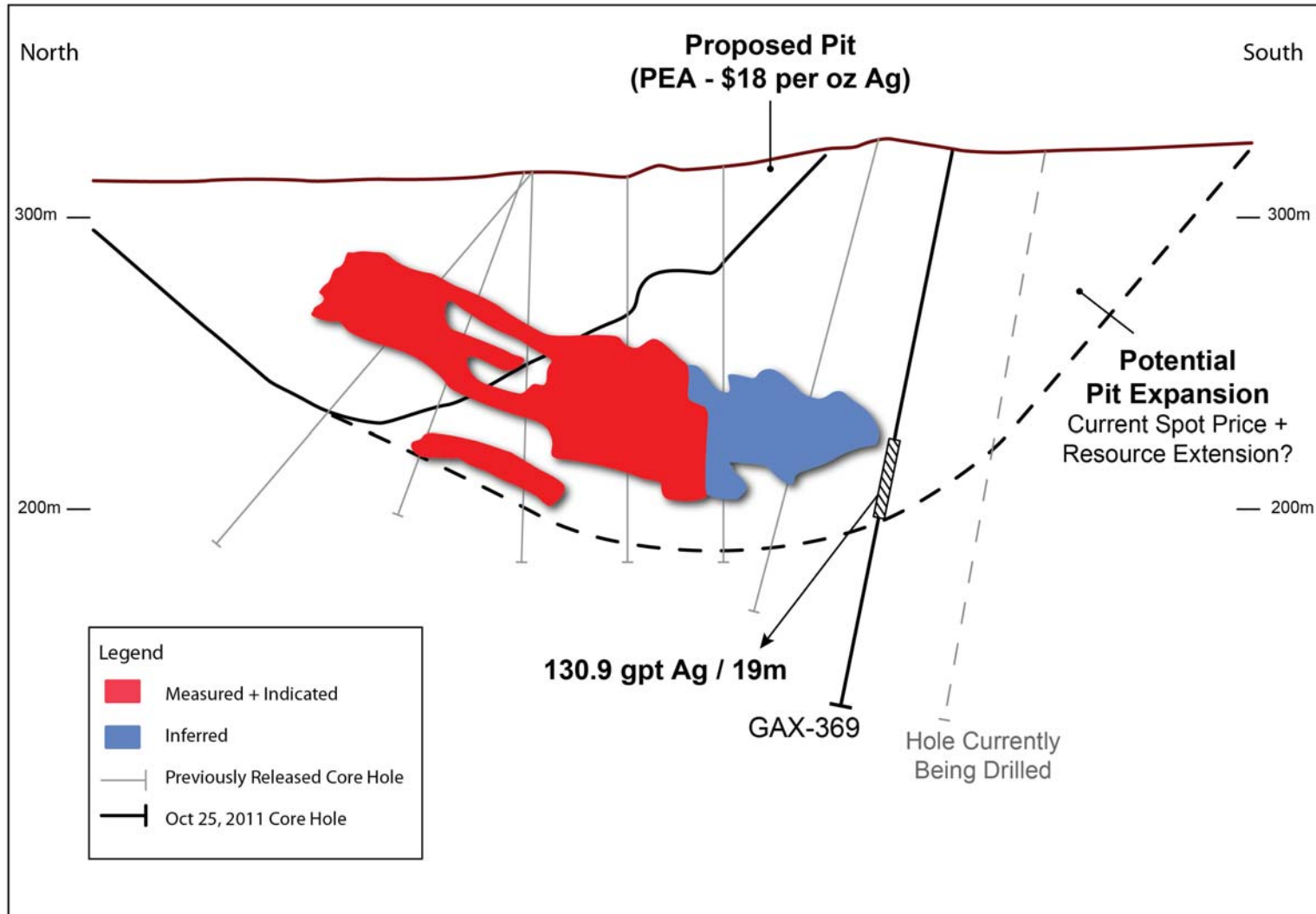
Figure 3 Cross Section View - Main Zone 28
