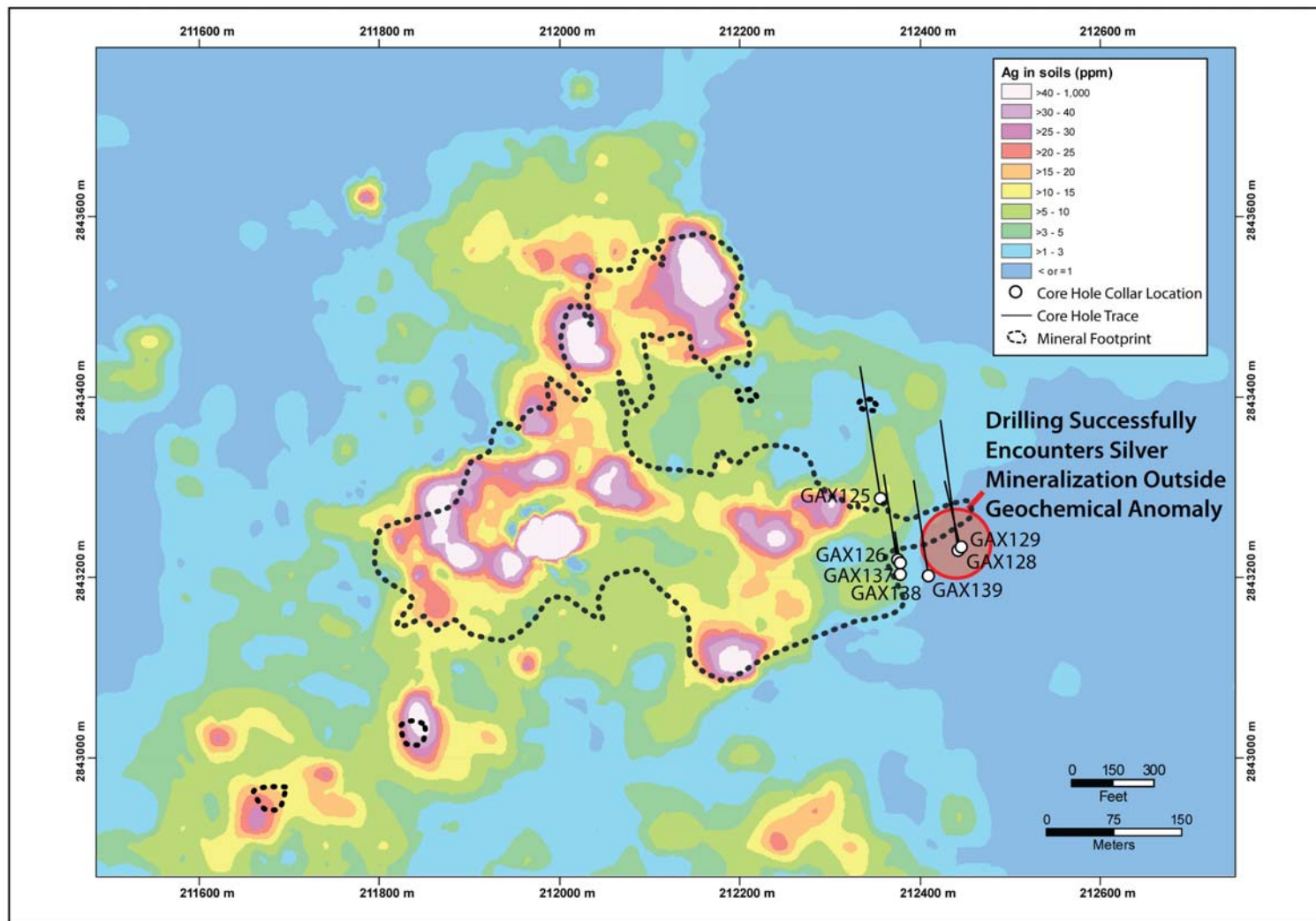
Figure 5 El Gallo Geochemical Soil Survey Signature – Plan (Aerial) View
