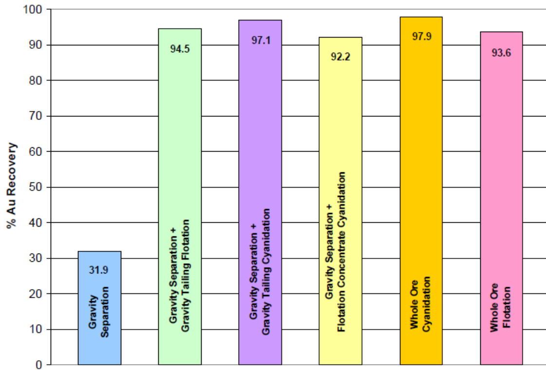
Figure 1 – Sample A – Comparison of overall flow sheet recoveries
