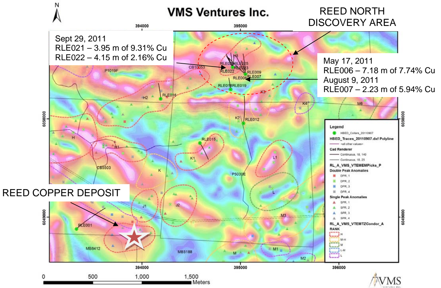
Figure 2. VTEM Anomalies with Magnetic Tilt
