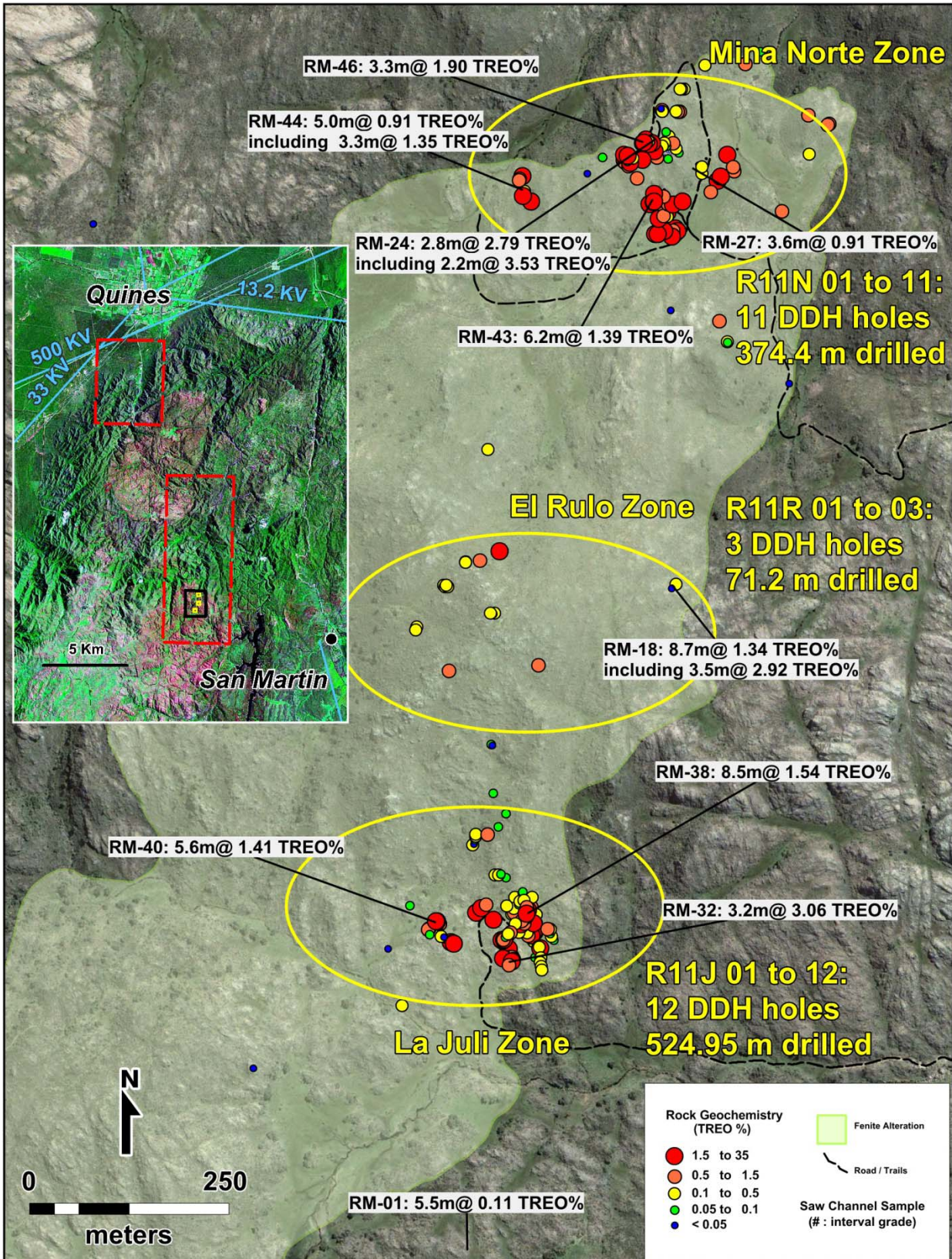
Figure 2: Map showing location of known zones of mineralization with surface results to date. Detailed maps of the La Juli and Mina Norte zones are available on the Company's website.
