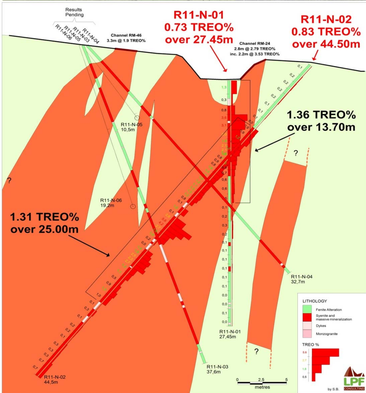
Figure 1: Plan and cross-section highlighting distribution and continuity of REE mineralization within the drill holes at the Mina Norte zone.
