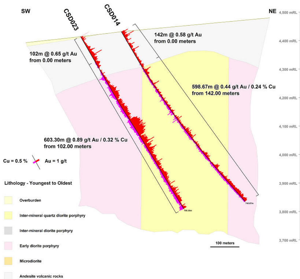
Figure 2 Drill section showing results and schematic geology for holes CSD014 and CSD023.
