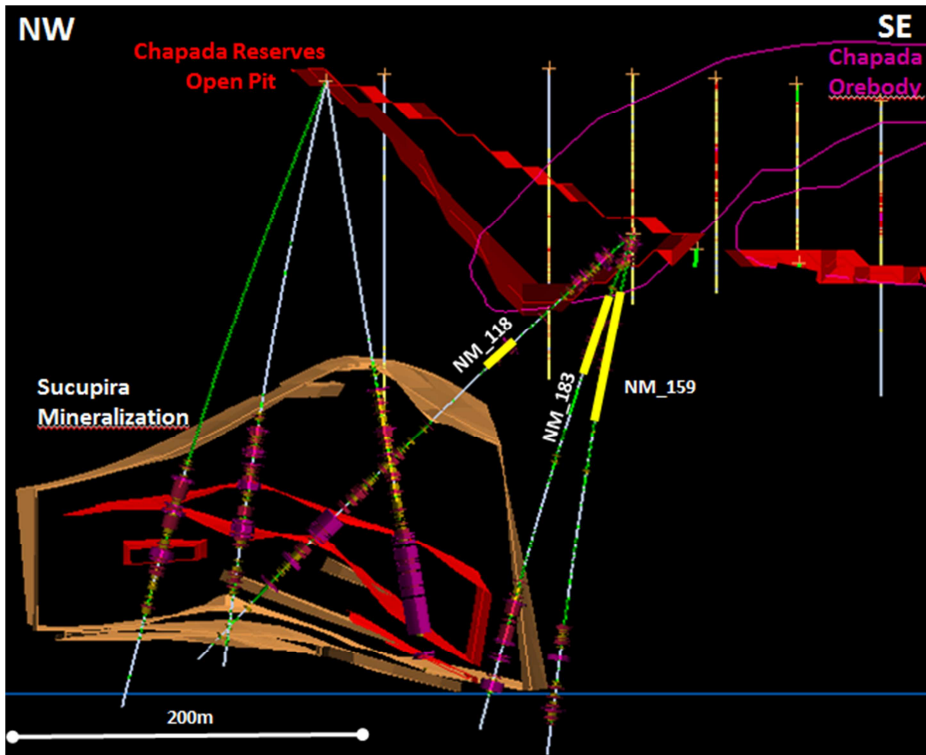
Figure 4: The figure above is a cross section view of the Chapada Open Pit with depictions of the Sucupira mineralization and mineral intercepts in yellow highlights superimposed on the drill hole traces beneath the pit.
