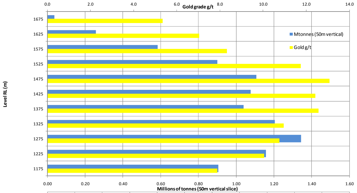
Yaragua Tonnes and Grade (> 3g/t Au) vs Elevation
