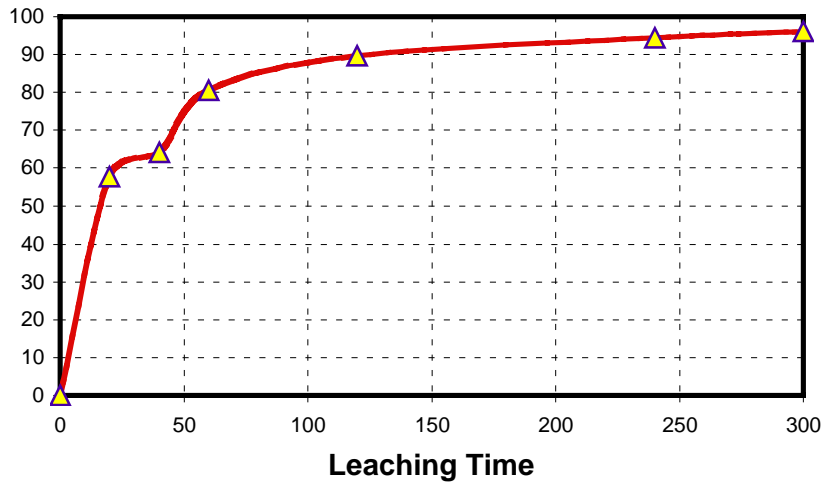
Rolled Bottle Test - Area 2
