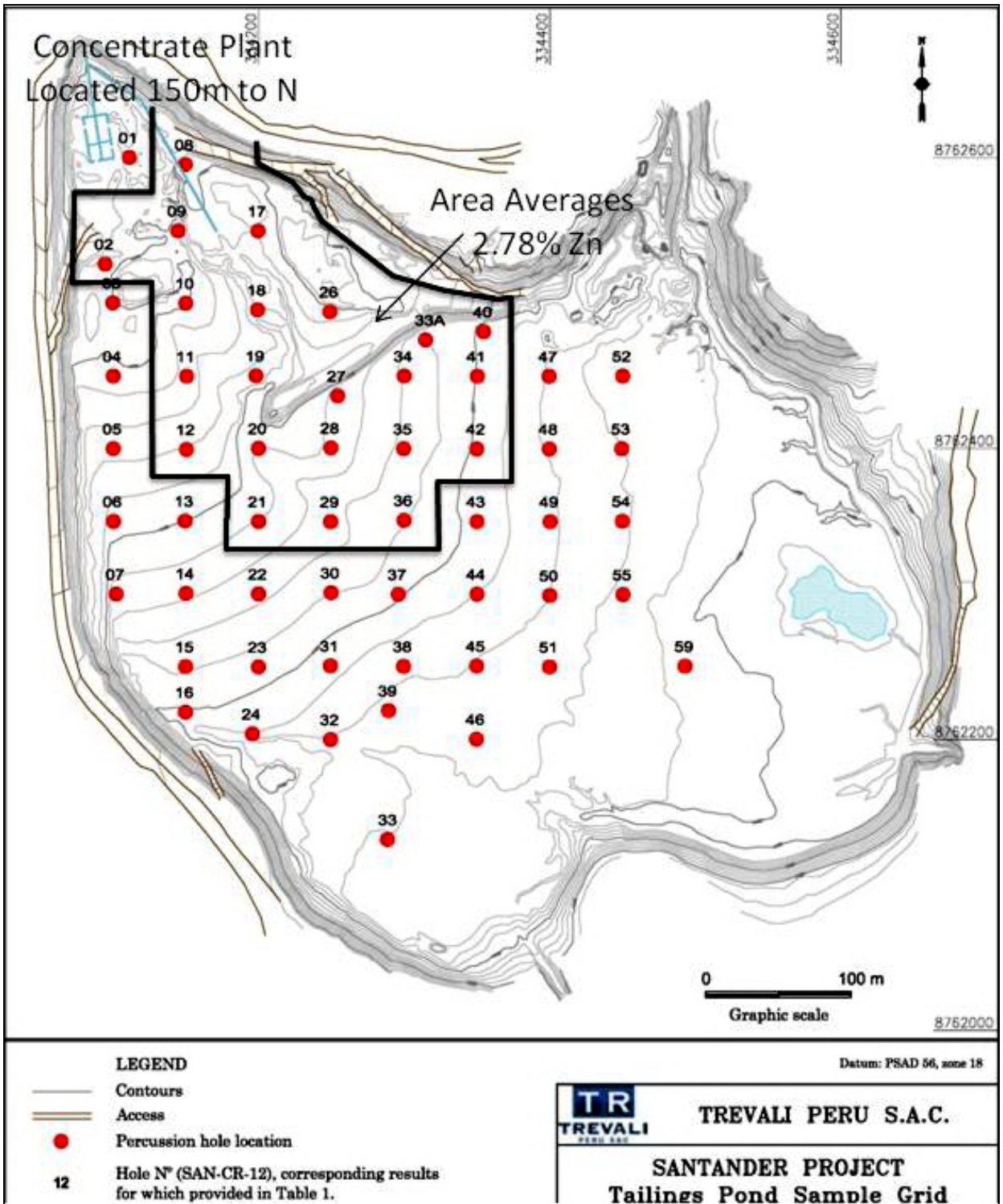
Figure 1: Summary borehole location map of Santander Tailings
