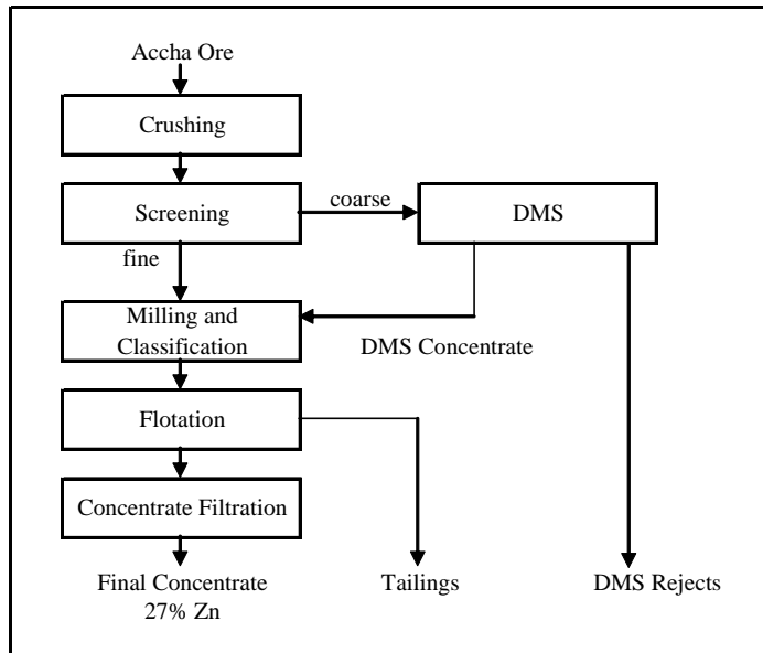
Figure 1 Simplified Process Diagram for the Accha Concentrator
