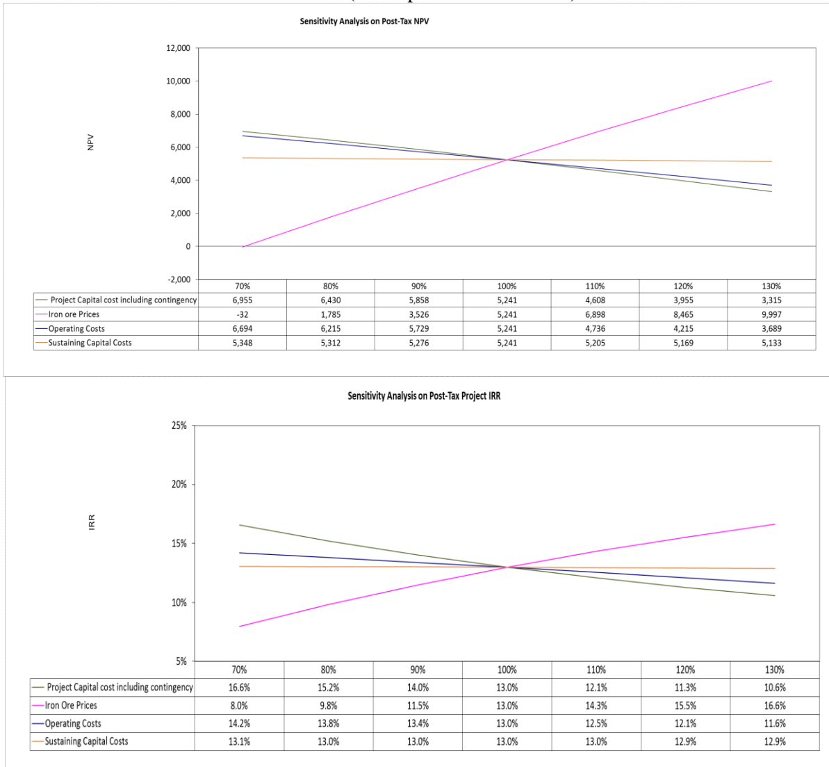
Figure 1 – Sensitivity of Post-Tax Project IRR and NPV to Key parameters Base Case (100% production to China)
