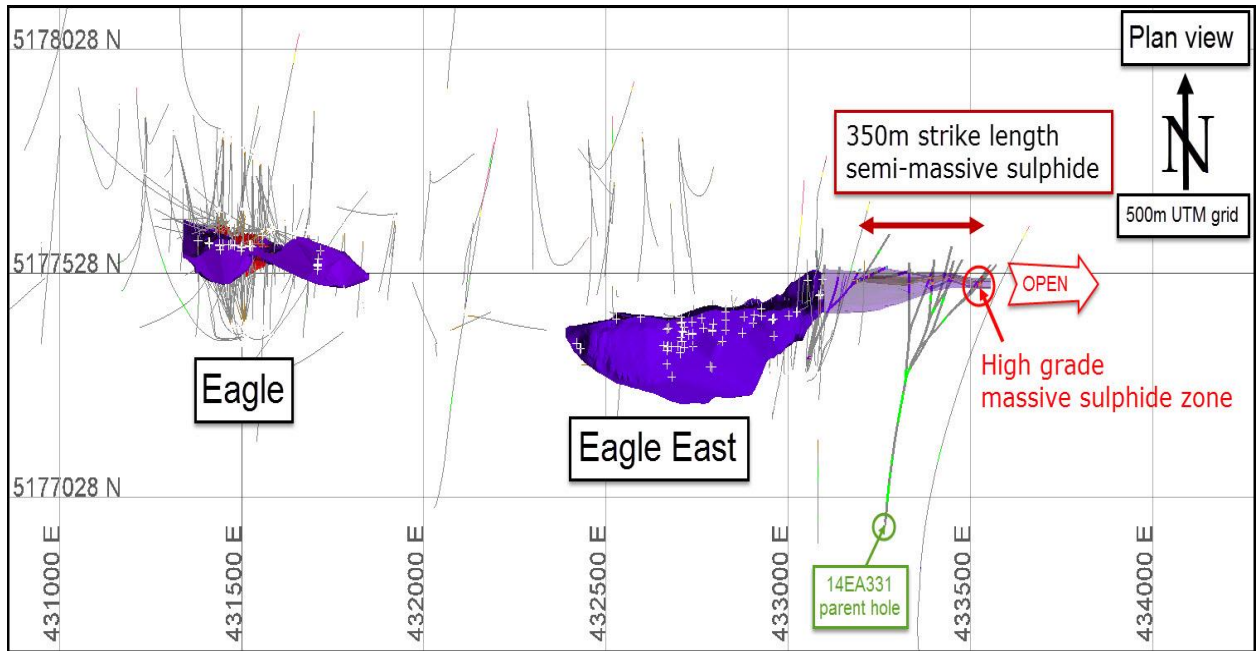
Figure 1. Plan view of Eagle and Eagle East modeled ultramafic intrusions (purple)
