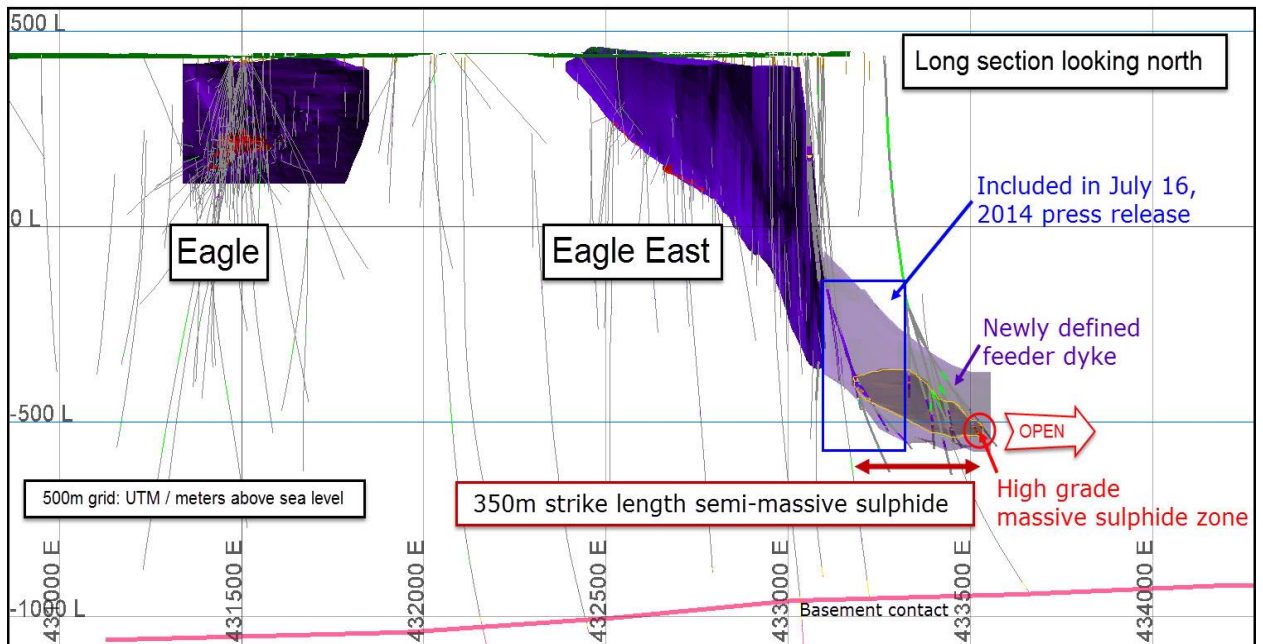
Figure 2. Long section of Eagle and Eagle East modeled ultramafic intrusions (purple)
