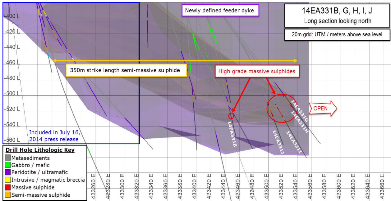
Figure 3. Detailed long section with drill holes
