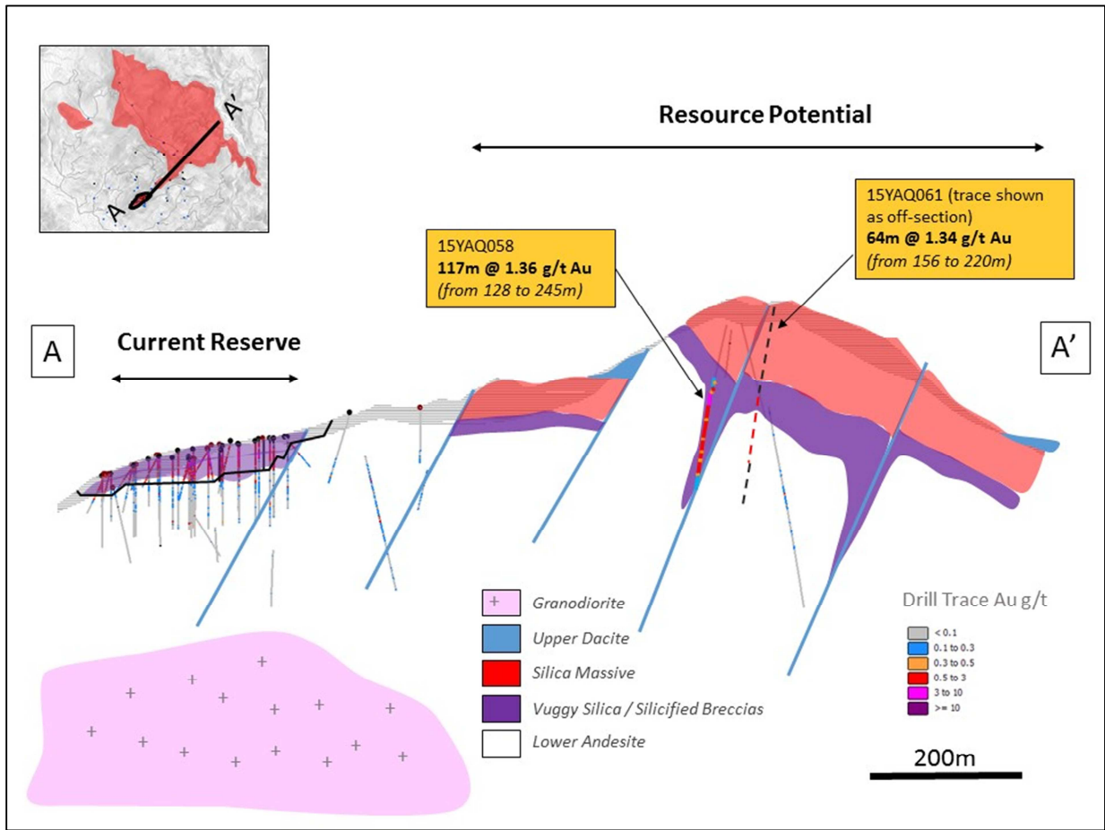
Figure 4: Greater Yaqui Project Area – Conceptual Long Section (Looking NW)
