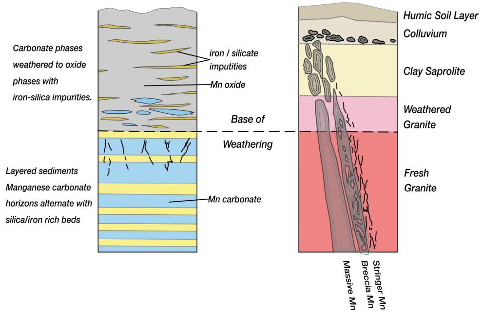
Comparison between sedimentary manganese and structurally-controlled manganese deposits.
