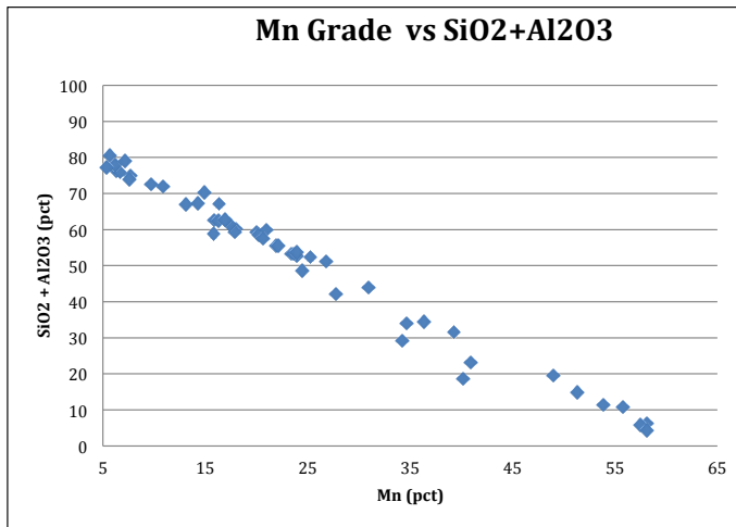
Plot of Mn vs. (SiO 2 +Al 2 O 3 ) for assay results received to date, showing the relationship between manganese grade and silicate content related to the host granite (left). DDH_J3_001 intersection (right), showing high-grade massive manganese with marginal lower grade breccia zone. Sample boundaries in orange.
