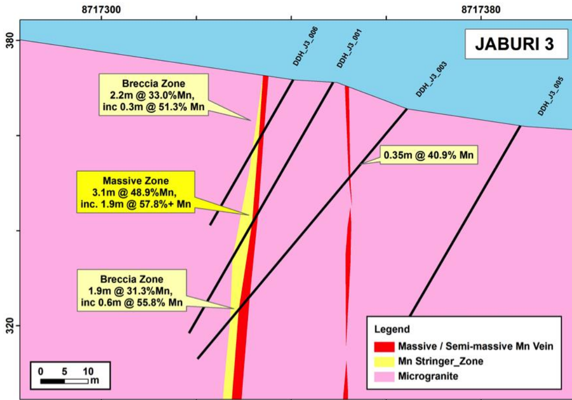
Jaburi 3 Cross Section
