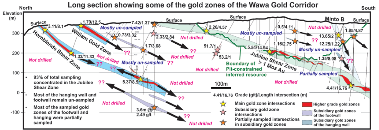
Figure 2 -- Oblique (173.5°) section showing extensive mineralization between the Shear and Gold Zones
