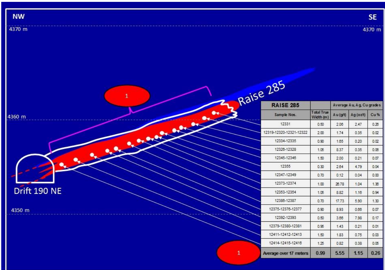
Figure 4. Cross-sectional view of Raise 285 Manto Dorado
