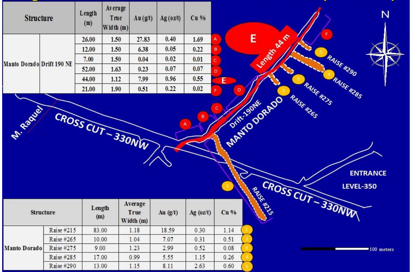
Figure 1. NE Plan View of the Manto Dorado (Level 350)
