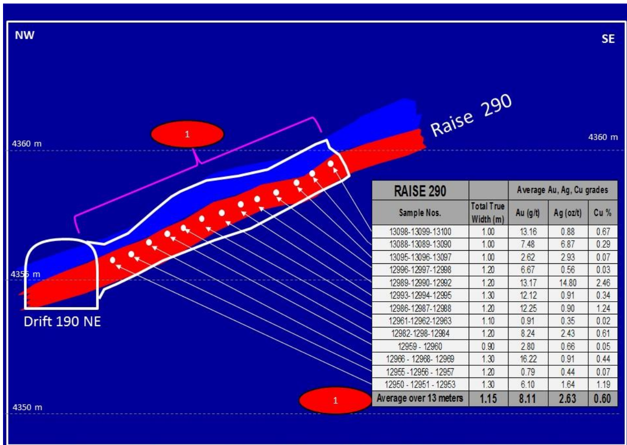
Figure 5. Cross-sectional view of Raise 290 Manto Dorado
