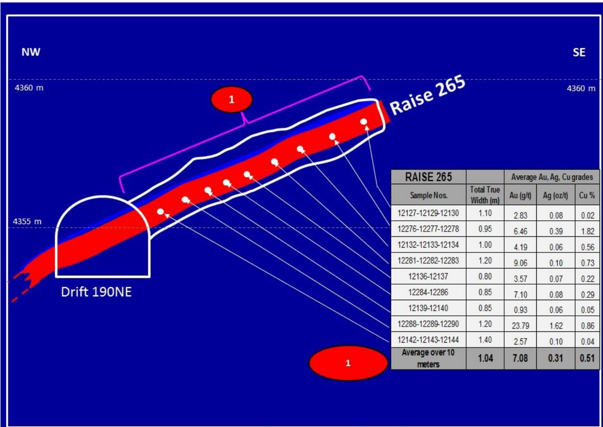
Figure 2. Cross-sectional view of Raise 265 – Manto Dorado
