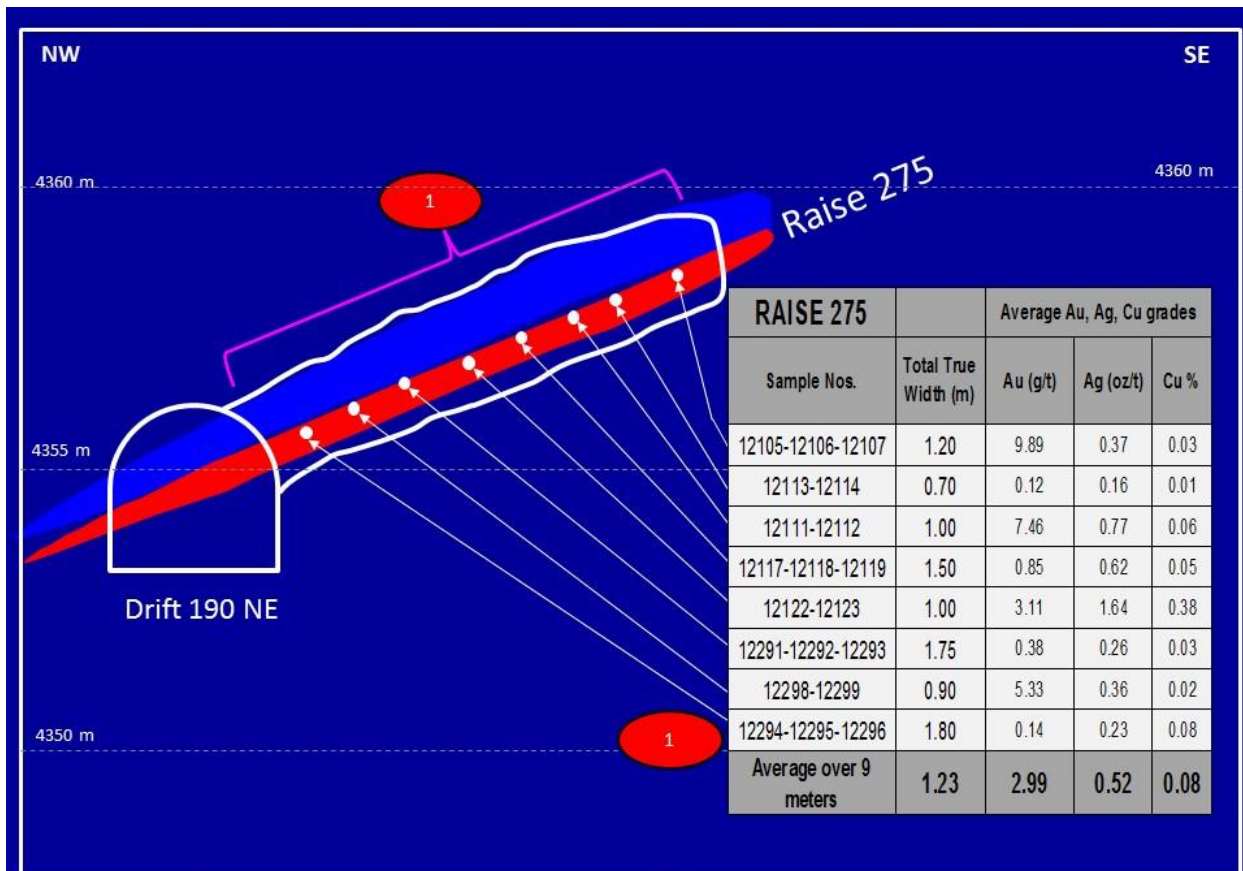
Figure 3. Cross-sectional view of Raise 275 – Manto Dorado
