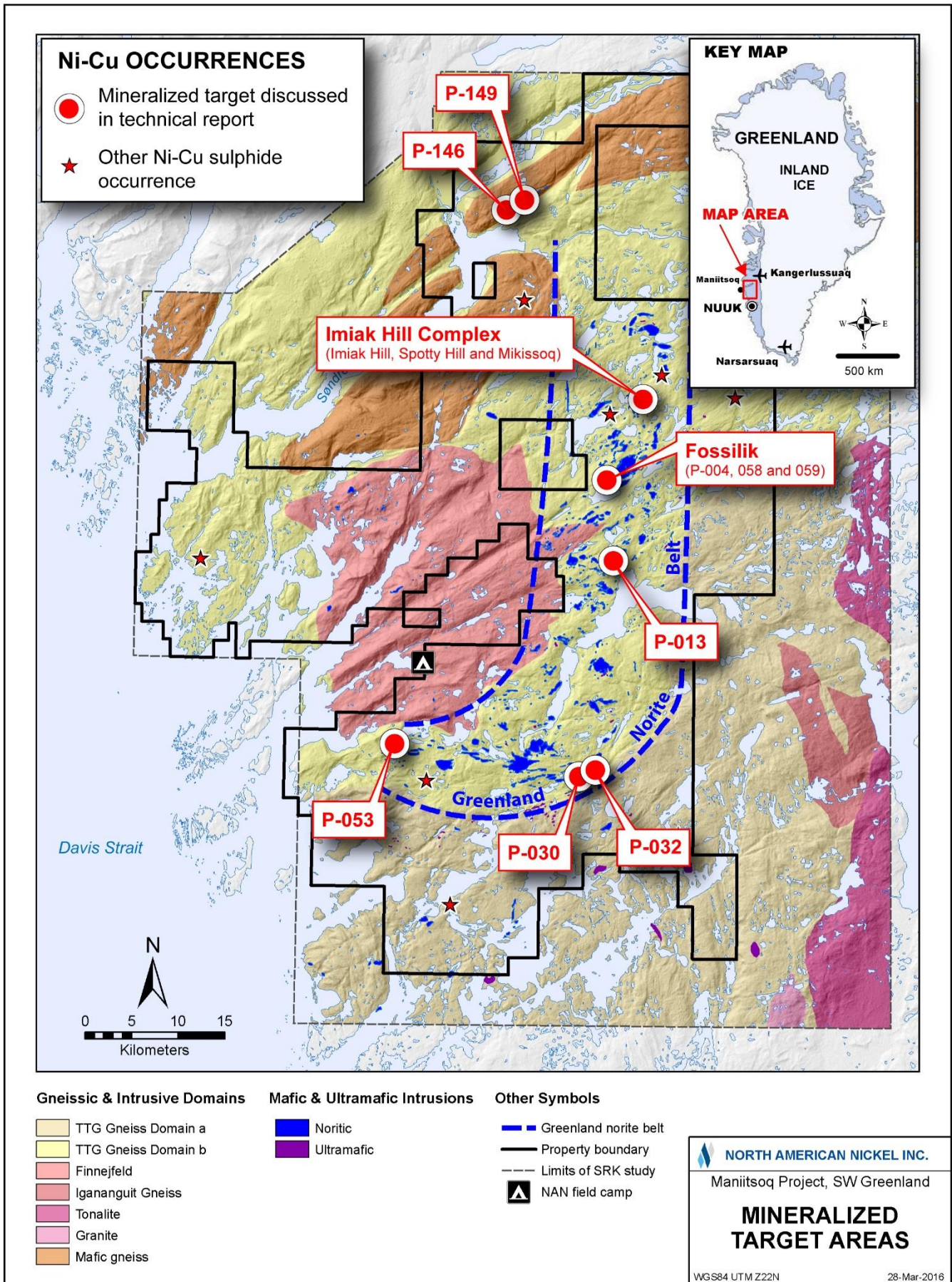
Figure 1: Location of Mineralized Target Areas, Maniitsoq Project, Greenland.
