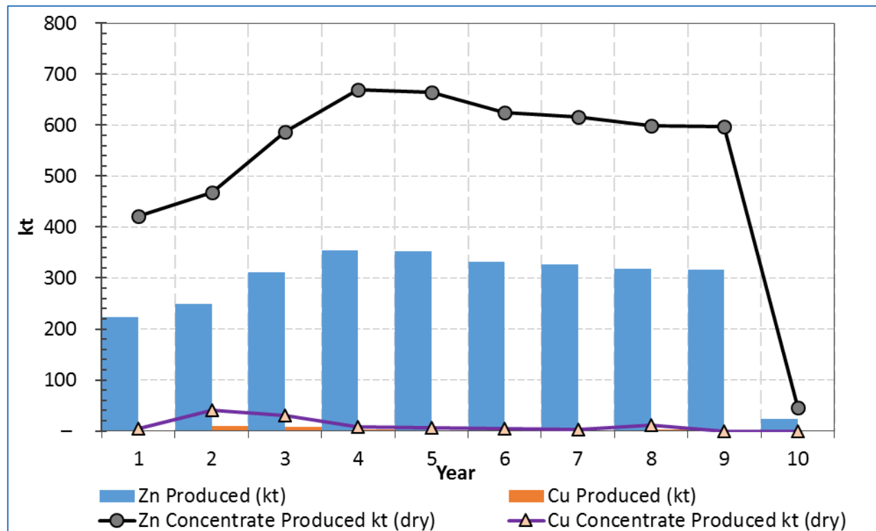
Figure 8: Concentrate and metal production
