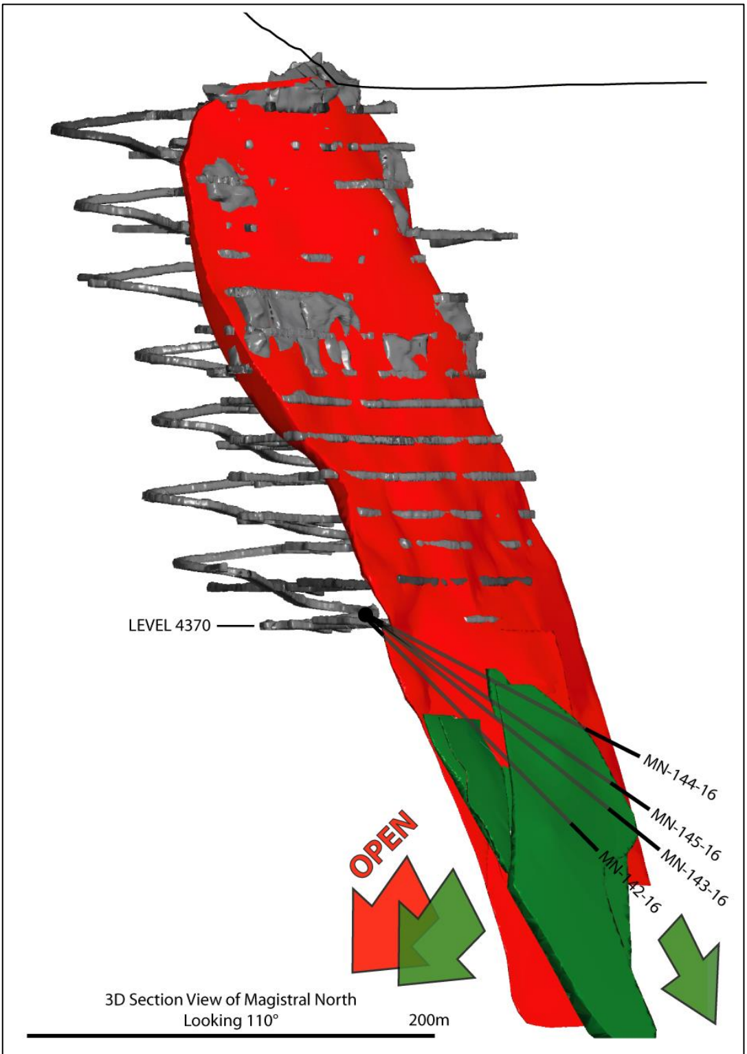
Figure 1: 3D view, looking southeast, and cross section illustrating geometry of the Oyon mineralization and location of recent drillhole intercepts in the Magistral North Deposit at the Santander Mine.
