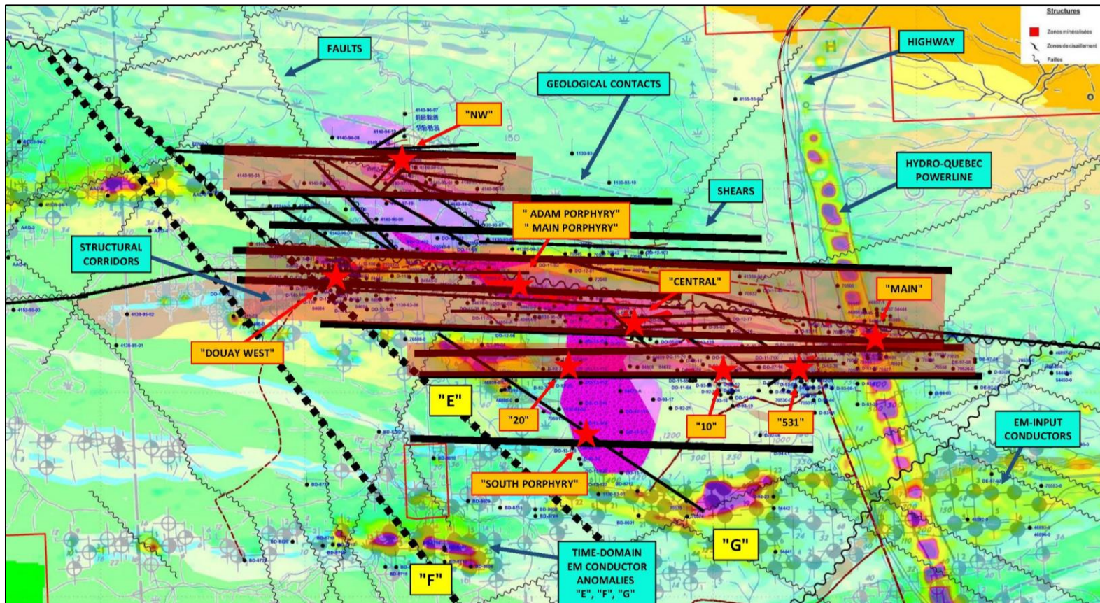
Figure 2. Predictive modeling from the Detailed Targeting Program showing the association between known gold occurrences and gold bearing shears and structural domains. North is towards top of the map. Dimensions are 10 km E-W and 6 km N-S. There are currently 9 identified E-W trending gold bearing shears and 3 major E-W structural domains of unknown extent at this time. Several higher grade gold zones appear at junctions of NW-SE, NE-SW and E-W shears; but at this time there is yet to be a link made between the gold mineralization and the junctions.
