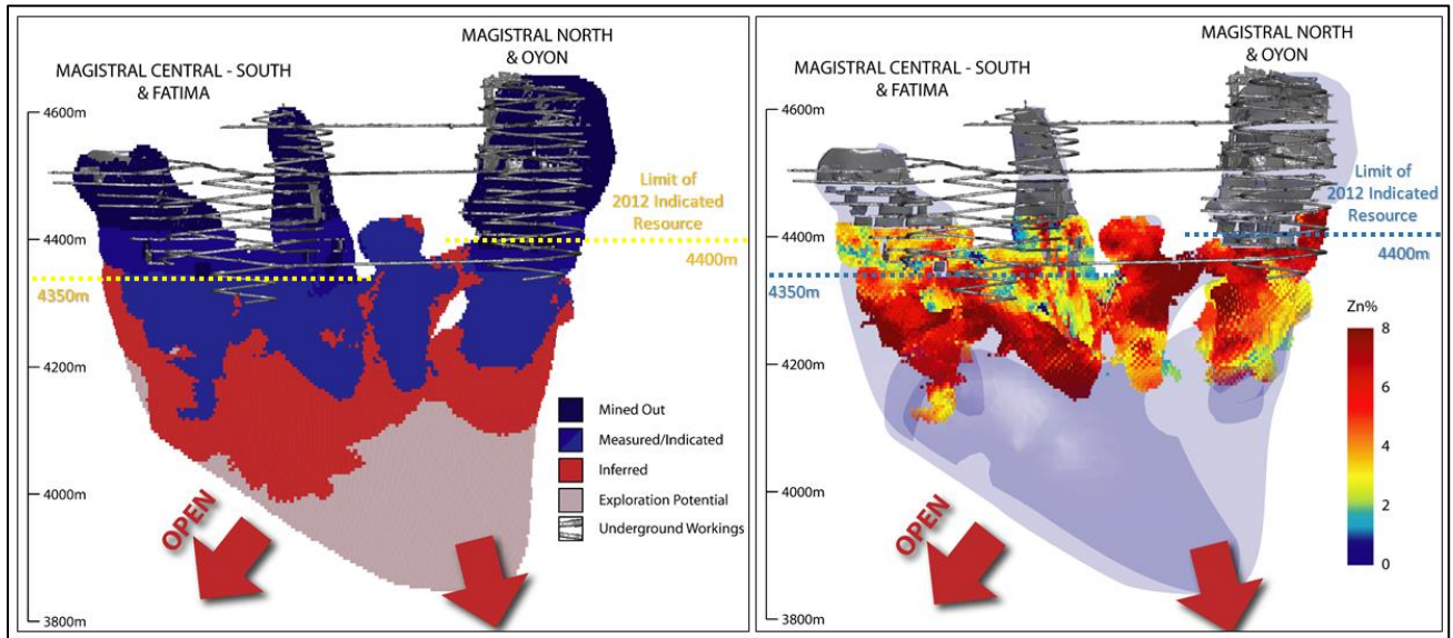
Figure 4: Long-section view, looking west, of the 2017 Magistral Deposits block model classification (Left) and zinc grades of the measured and indicated blocks (Right).
