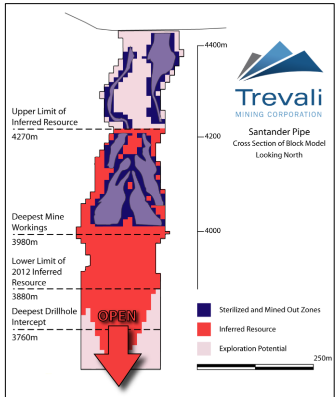
Figure 5: Santander Pipe model (left) and a section (right) illustrating location of currently defined Inferred Resources and formerly mined areas. Mineralization remains open for expansion at depth.
