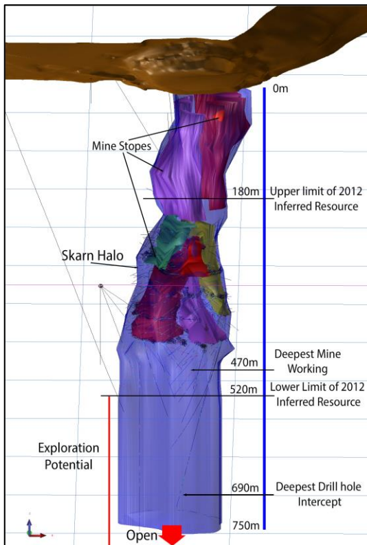
Figure 5: Santander Pipe model (left) and a section (right) illustrating location of currently defined Inferred Resources and formerly mined areas. Mineralization remains open for expansion at depth.
