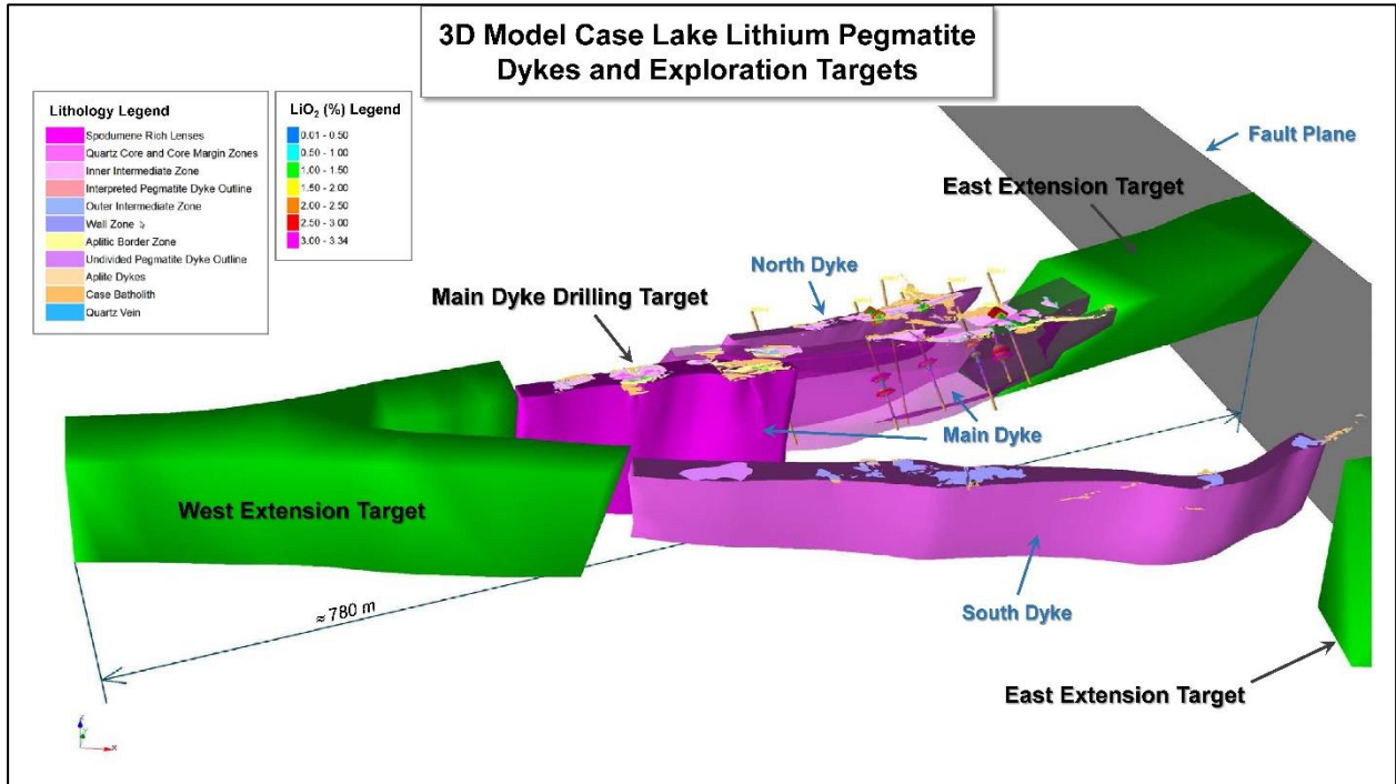
Figure 1 3D model of Case Lake North, Main and South Dykes and exploration targets, looking north.
