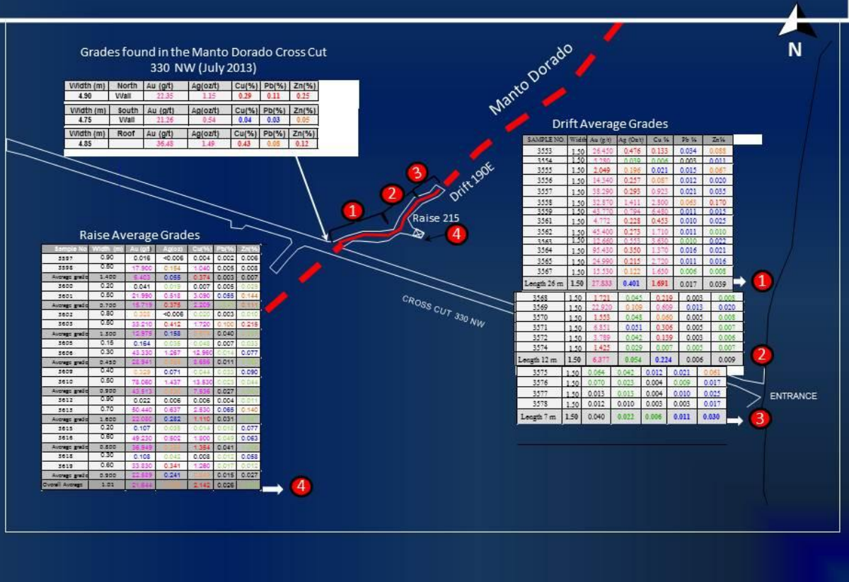
Figure 2 Underground Excavation Plan View, Cross Cut, Drift and Raise, Manto Dorado, Tumipampa.
