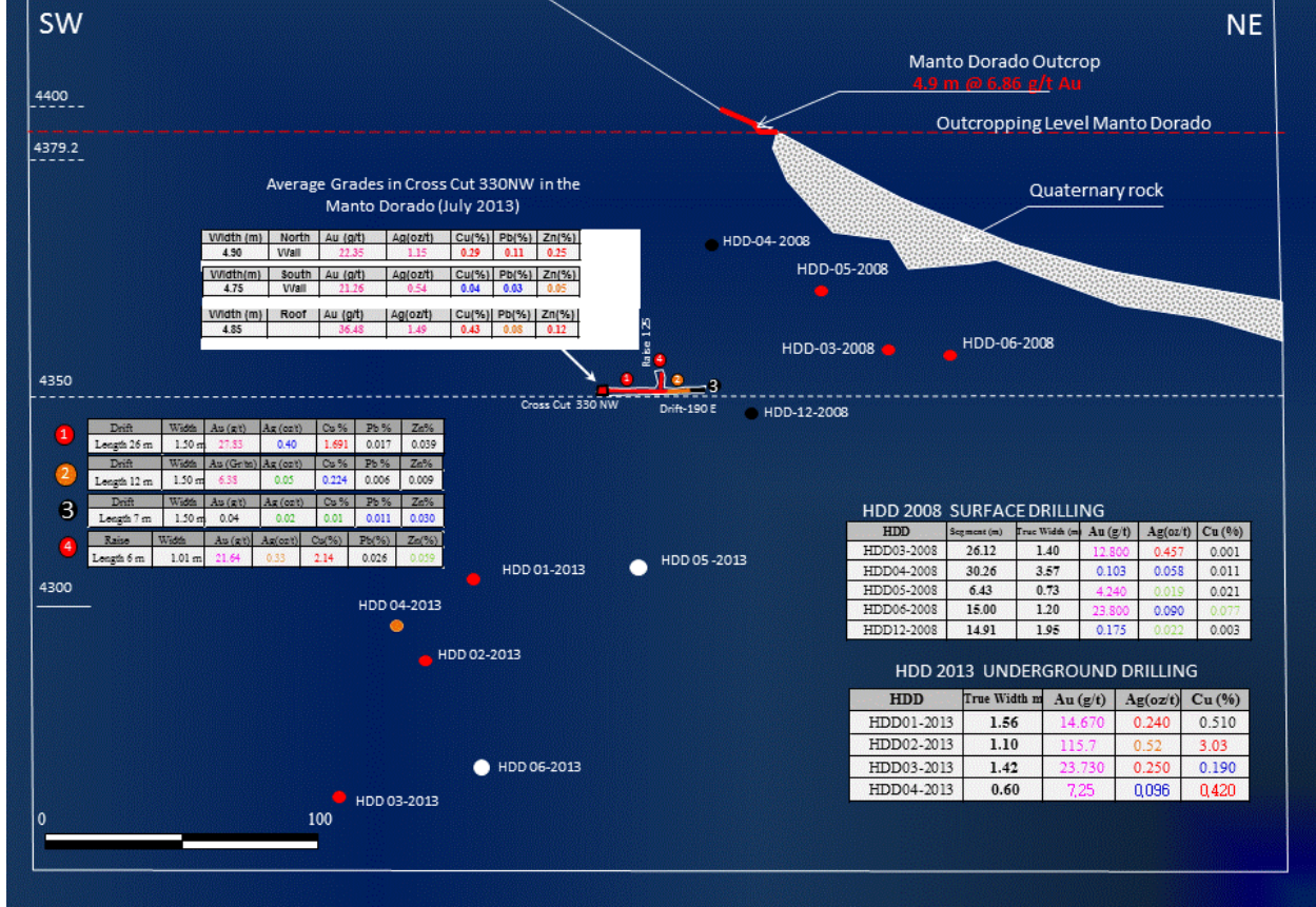
Figure 3. Longitudinal Section of Drilling, Cross Cut, Drift and Raise and Sampling Results, Manto Dorado, Tumipampa.
