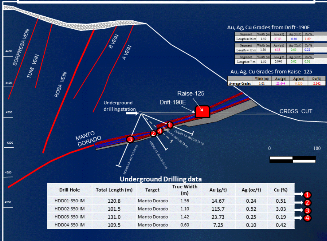
Figure 1. Underground drilling HDD01-2013 to HDD04-2013 in the Manto Dorado, Tumipampa
