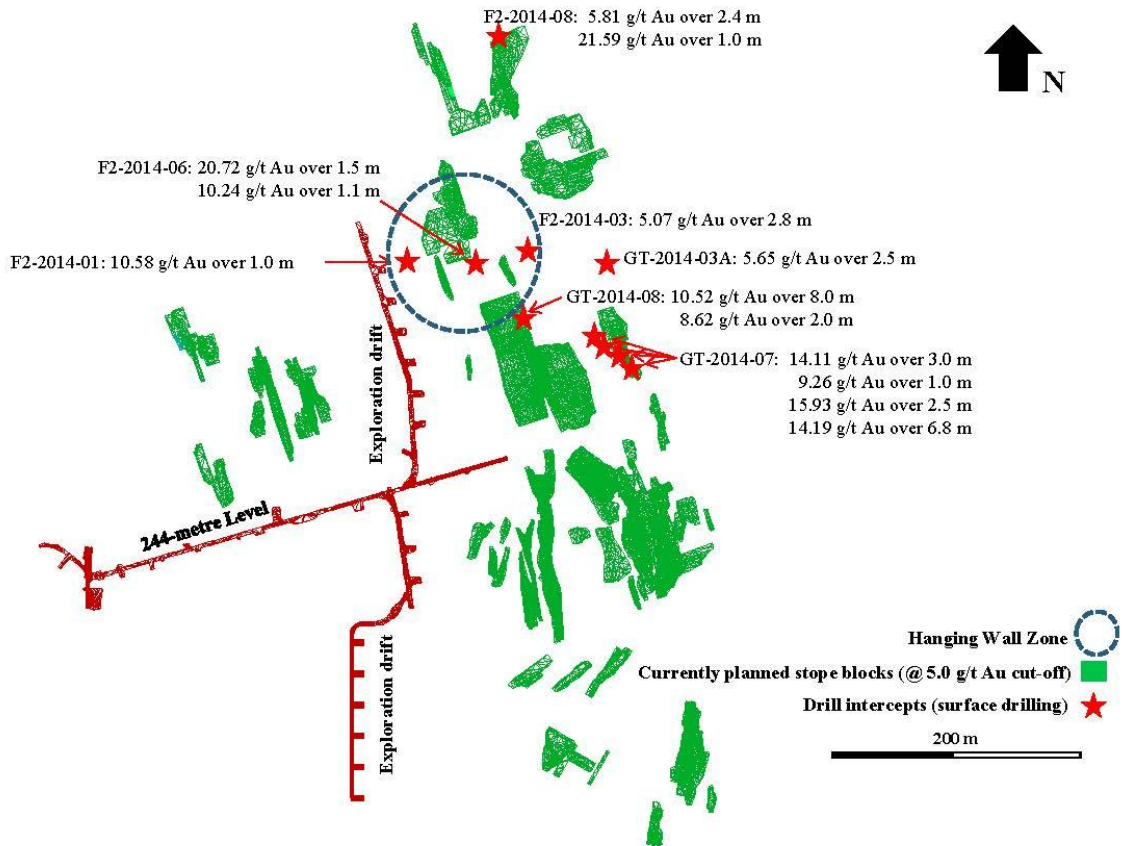
Figure 1: Plan View of the Infill Drilling Program (from Surface) Plotted Over Planned Stope Shapes
