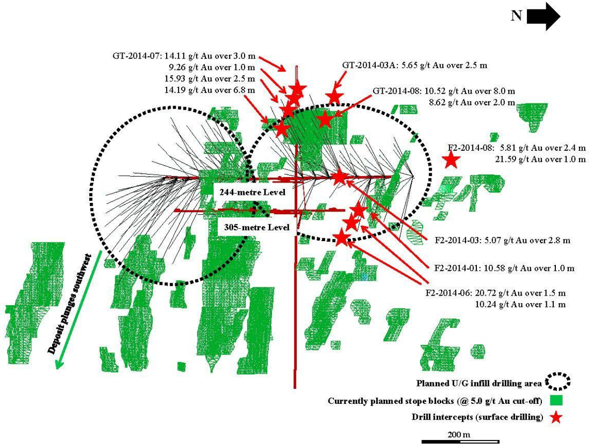
Figure 3: Long Section View of the Infill Drilling Program From the Surface Drilling Plotted Over Planned Slope Shapes
