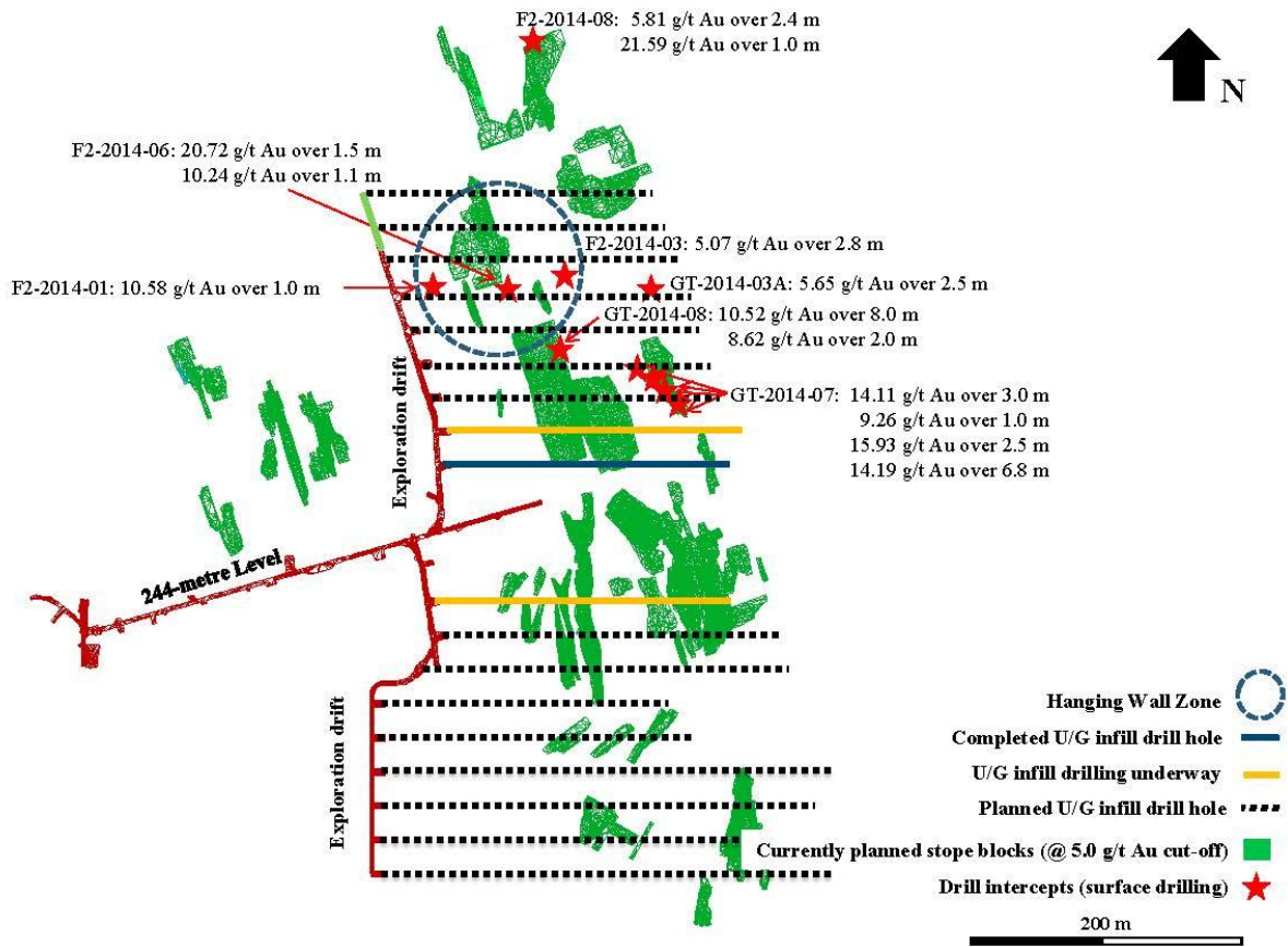
Figure 2: Plan View of the Infill Drilling Program Plotted Over Planned Stope Shapes
