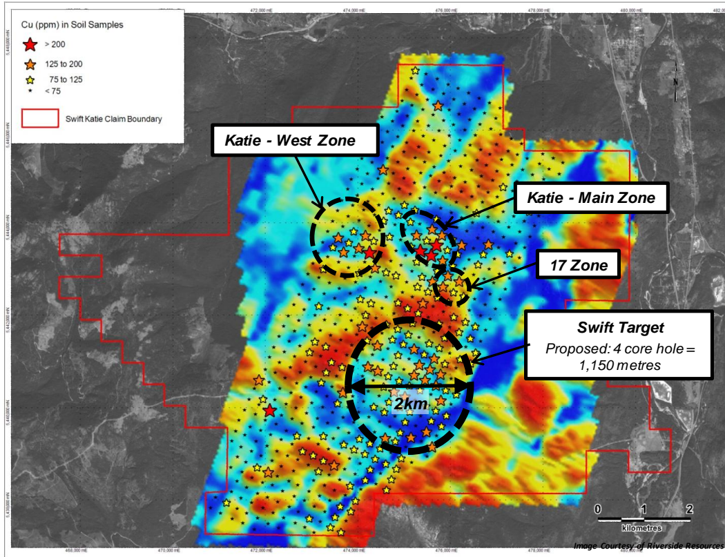
Figure: Airborne Resistivity, copper soil anomalies at the Swift Katie Project
